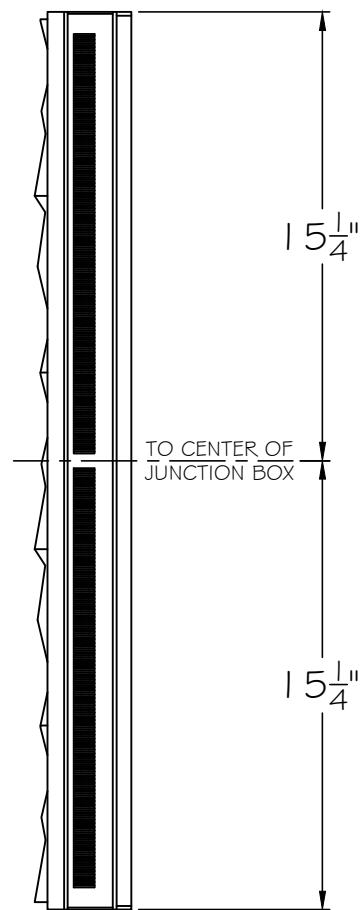
RIGHT VIEW
