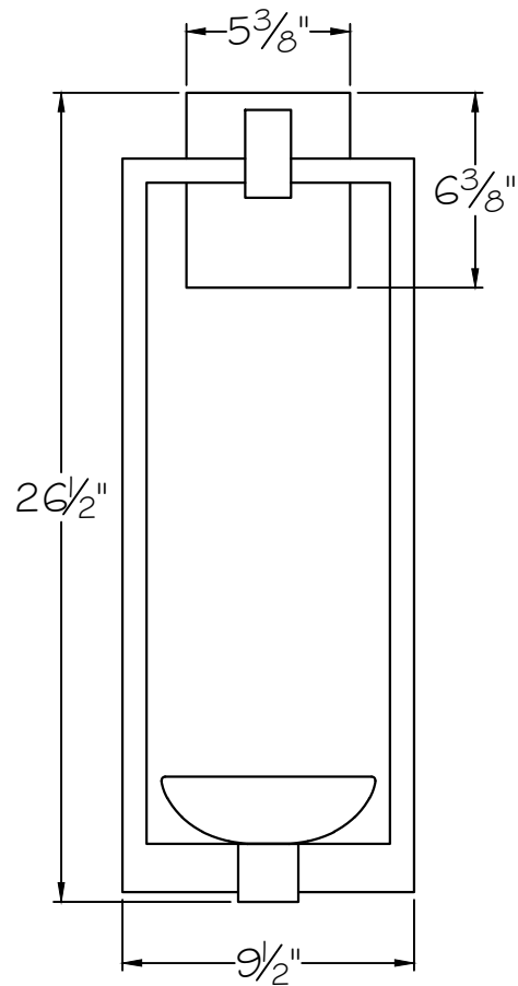
FRONT VIEW
