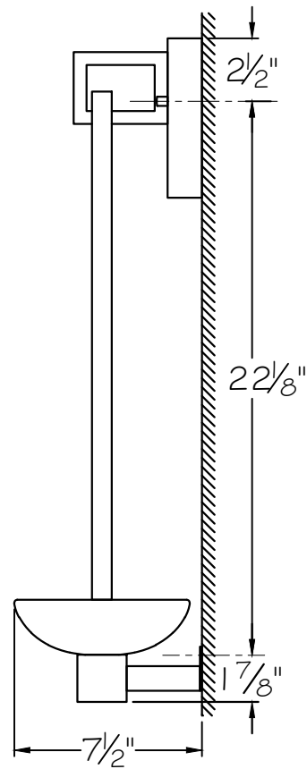
SIDE VIEW
