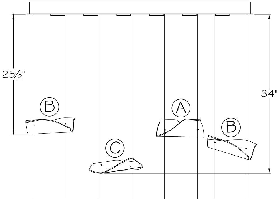
FRONT VIEW OF LAYER 1 GLASSES
