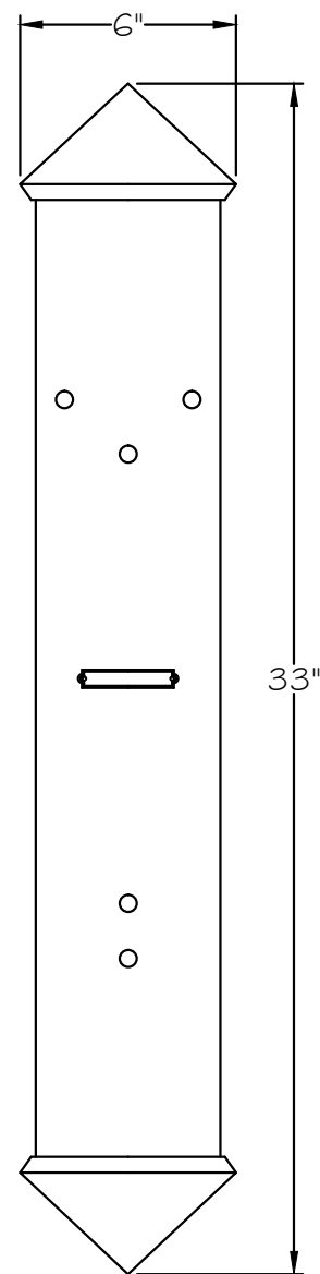
BACK PLATE
