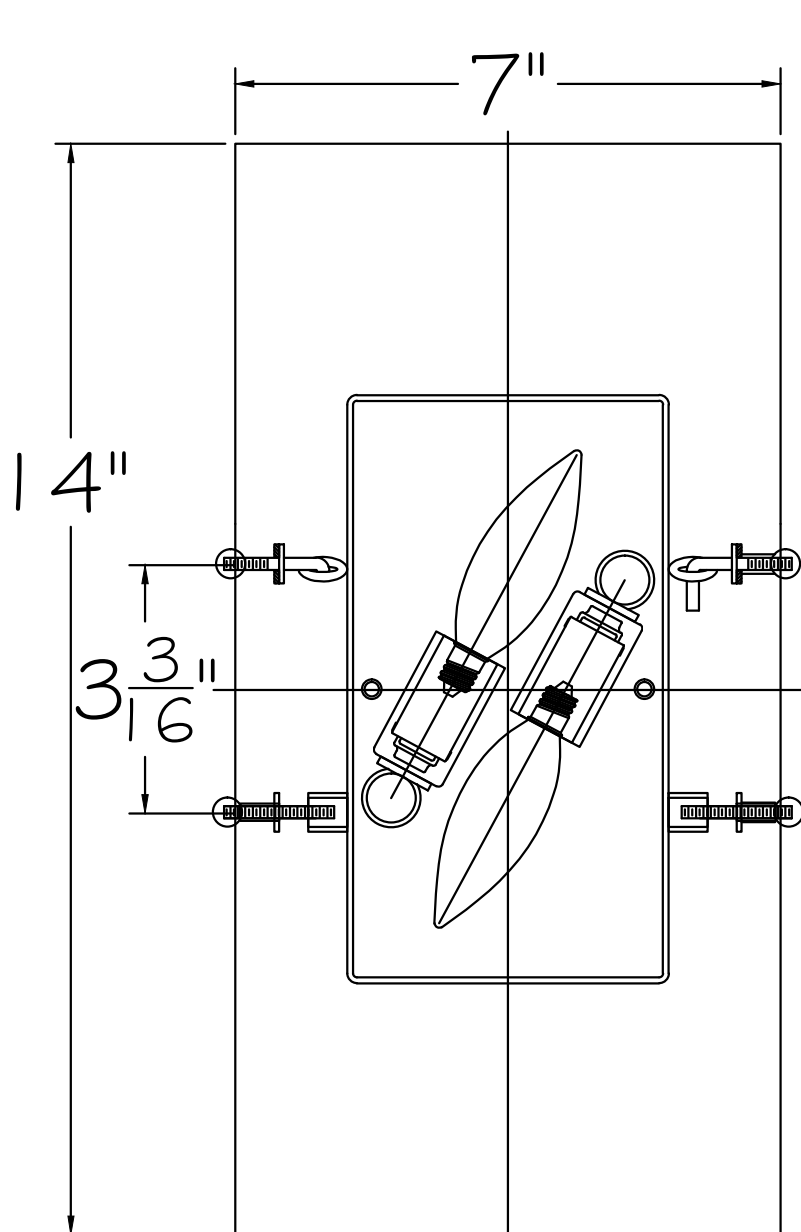
FRONT VIEW
