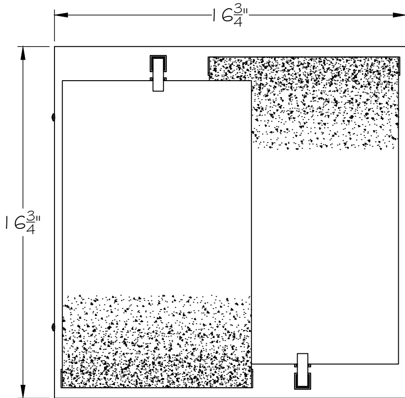
BOTTOM VIEW
