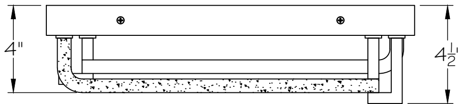
SIDE VIEW
