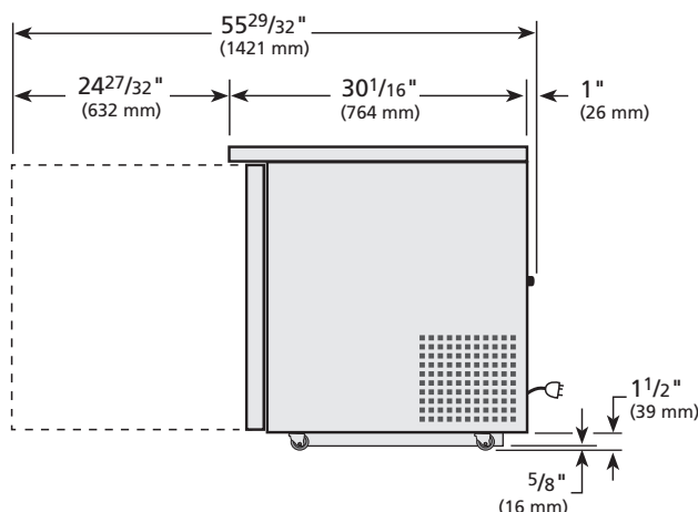
RIGHT VIEW
