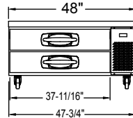
MBCB48 ELEVATION VIEW
