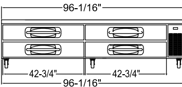
MBCB96 ELEVATION VIEW
