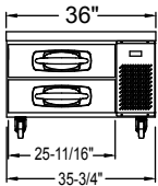
MBCB36 ELEVATION VIEW
