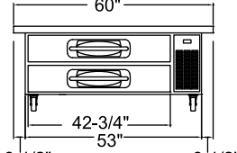
MBCB60 ELEVATION VIEW
