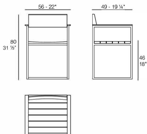
VINEYARD Silla VINEYARD Chair
