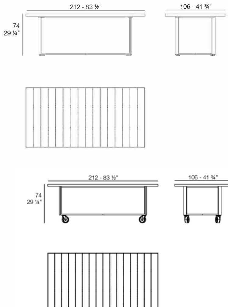
VINEYARD Mesa Comedor VINEYARD Dining Table
