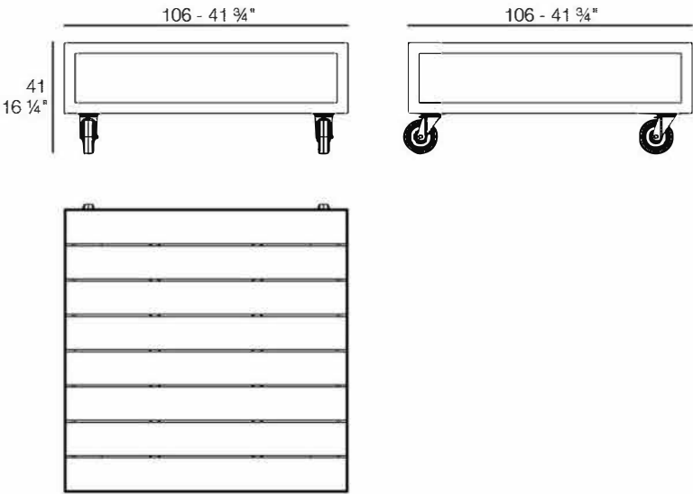
VINEYARD Mesa L VINEYARD Table L
