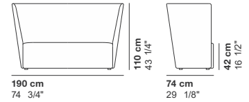
cod. 3502 / B_2 seater H.110
