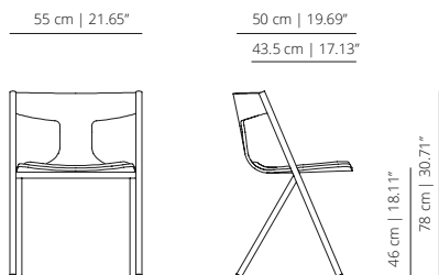
SKU:VIMOBÉ-401-QUARO chair with cushion
