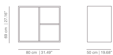
DO800DB storage unit 800 + dividers
