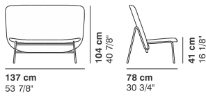
cod. 8890 / steel_small armchair
