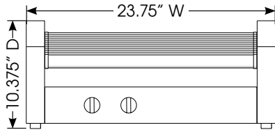
8033 - Front VIEW
