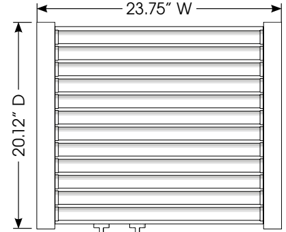
8033 - TOP VIEW
