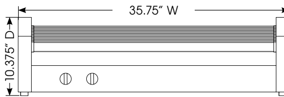
8055 - Front VIEW
