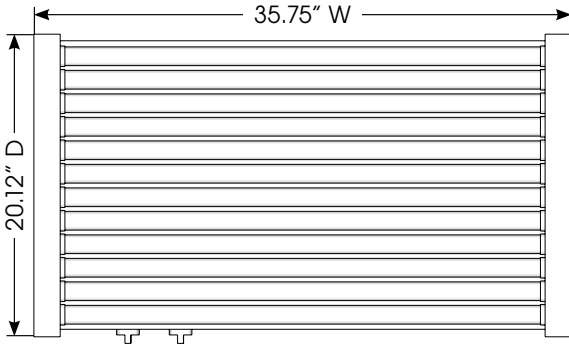
8055 - TOP VIEW
