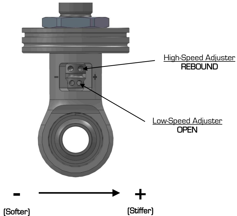
Figure 22b - Detroit Speed Recommended Settings
