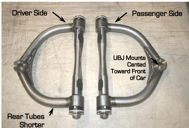
Figure 15 - Driver & Passenger Upper Control Arms
