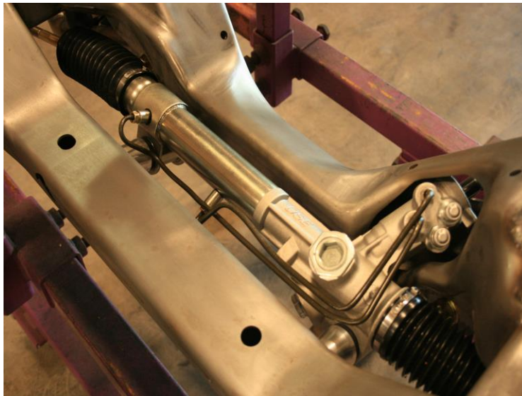
Figure 4 - Installed Rack
