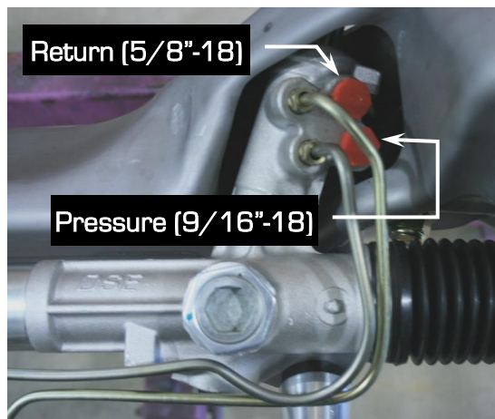
Figure 18 - Pressure and Return Port Locations
