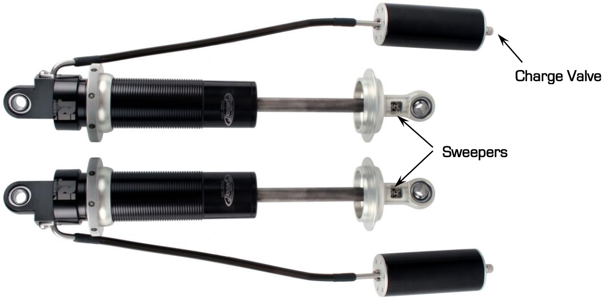
Figure 22a - Detroit Speed Double Adjustable Shock W/Remote canisters
