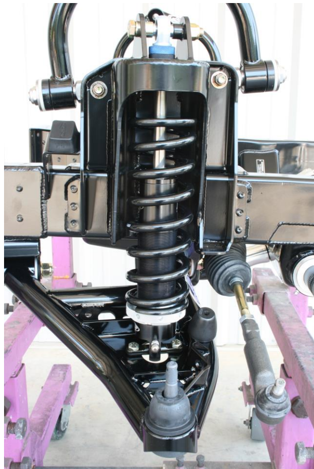
Figure 14 - Installed Coilover View
