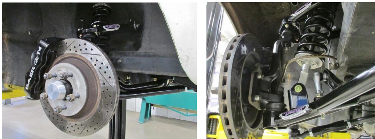
Figure 41 – Re-Install Brakes
