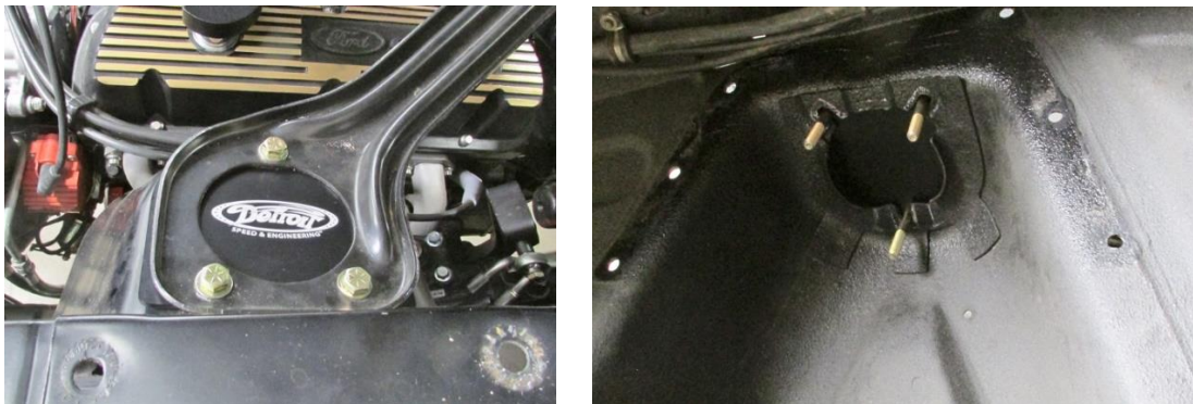
Figure 9 - Locate Strut Tower Brace Hardware
