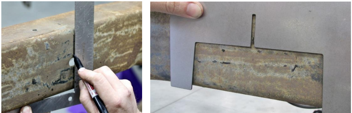
Figure 6 - Frame Notch Template
