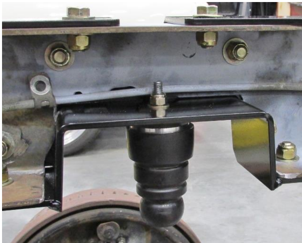
Figure 13 - Install Jounce Bumper
