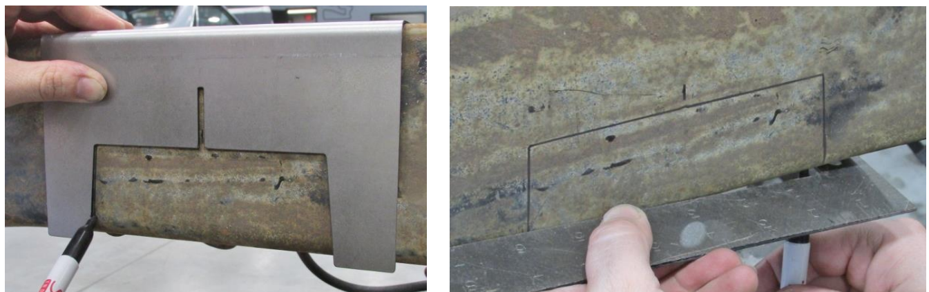
Figure 7 - Trace Frame Notch Cutout
