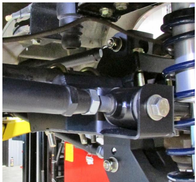
Figure 31 – Install Track Bar
