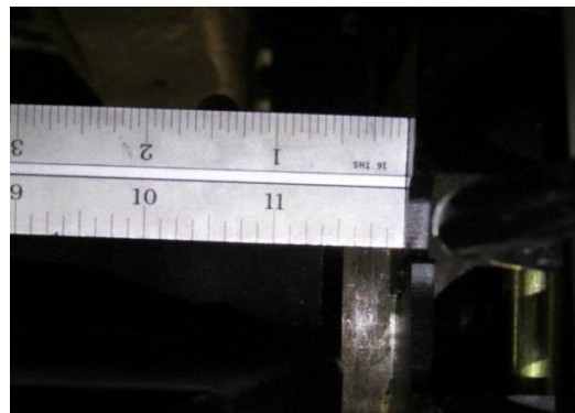
Figure 28 - Locate Track Bar Axle Bracket
