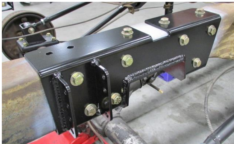
Figure 11 - Install Frame Notch Assemblies (LH, Driver Side)
