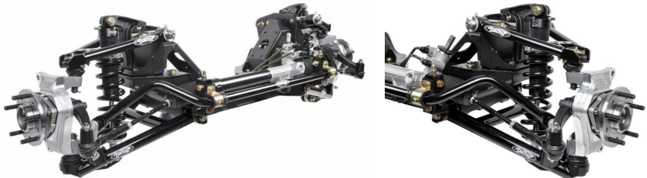
Figure 98 - Completed Installation
