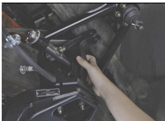
Figure 49 - Position Upper Coilover Mount
