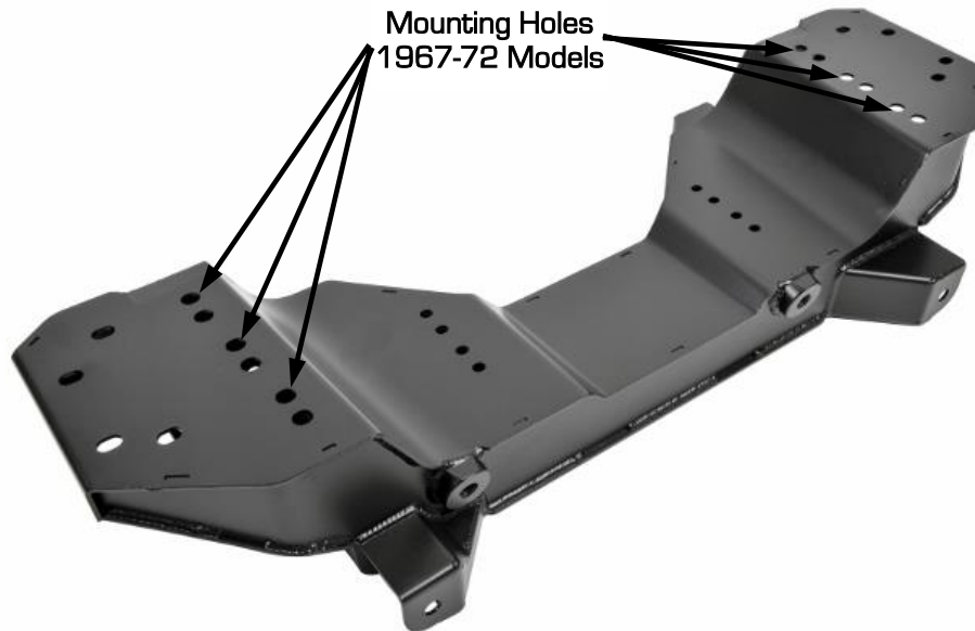
Figure 27 - DSE Cradle Assembly
