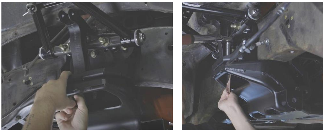
Figure 52 - Torque Upper Coilover Mount
