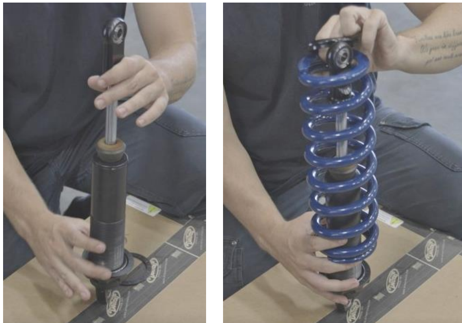
Figure 76 – Coilover Spring & Bearing
