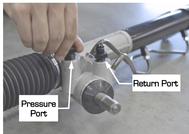
Figure 59 - Install Rack Fittings
