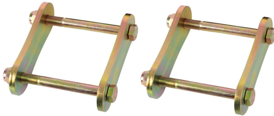
Figure 1 – PN: 041504DS, Heavy Duty Rear Shackles with Assembled Hardware
