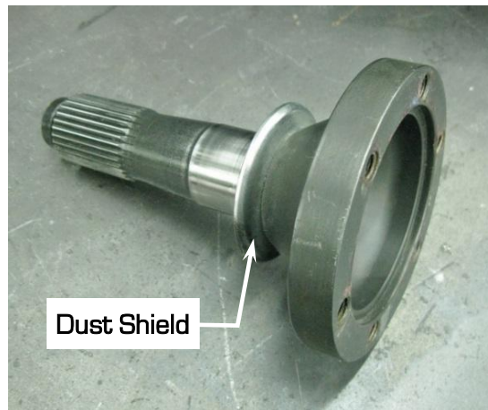
Figure 67 – Stub Axle Shafts
