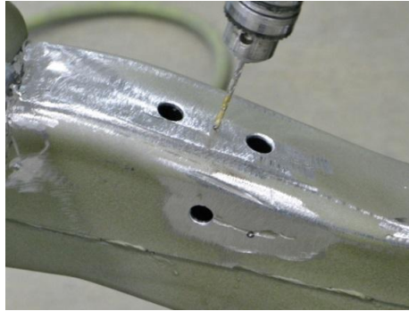
Figure 47 – Drill & Chamfer Nut Plate Locators
