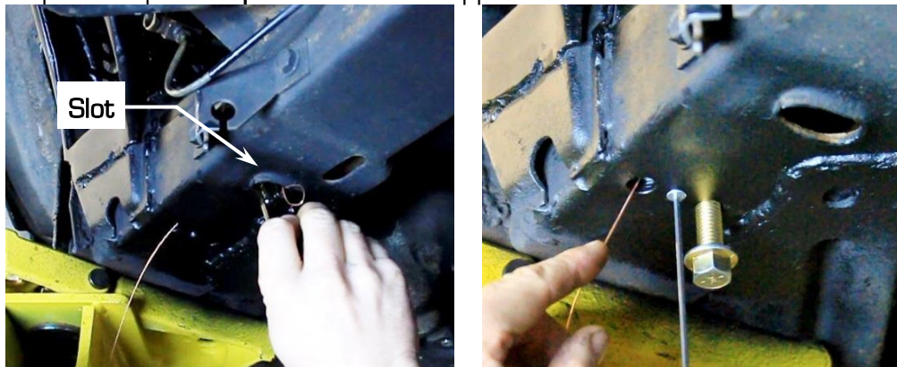
Figure 31 – Install Trailing Link Bracket Nut Plate
