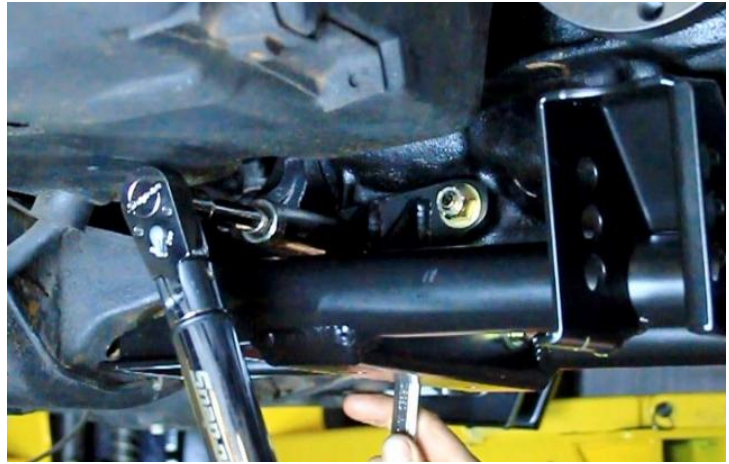
Figure 93 – Torque Lower Differential Bracket
