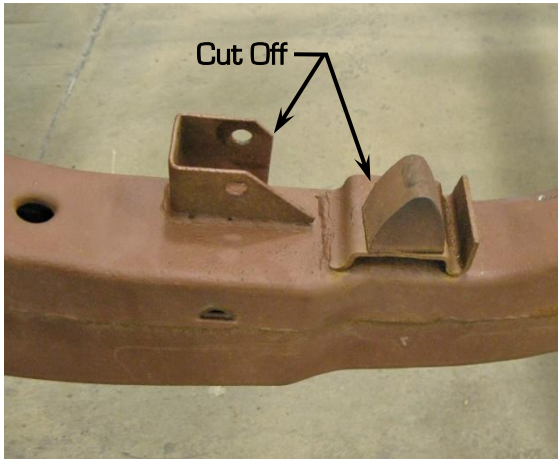
Figure 4 – Remove Frame Bumper and Upper Shock Mount Brackets
