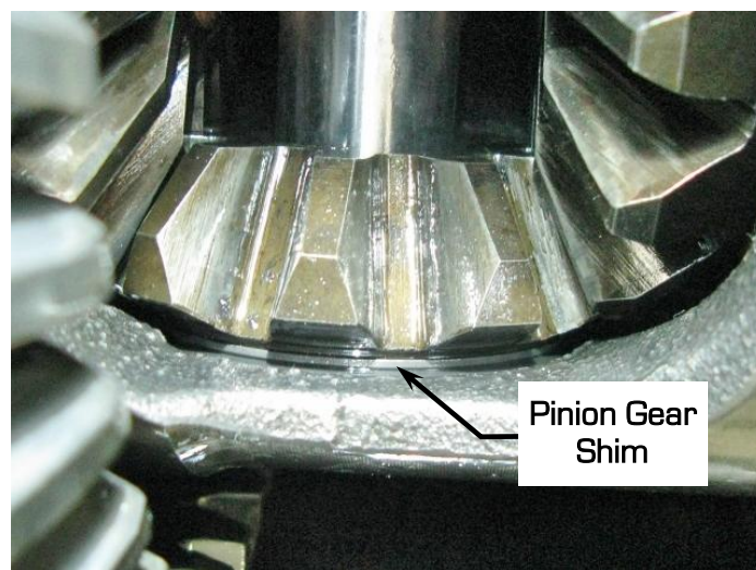
Figure 70 - Pinion Gear Shim
