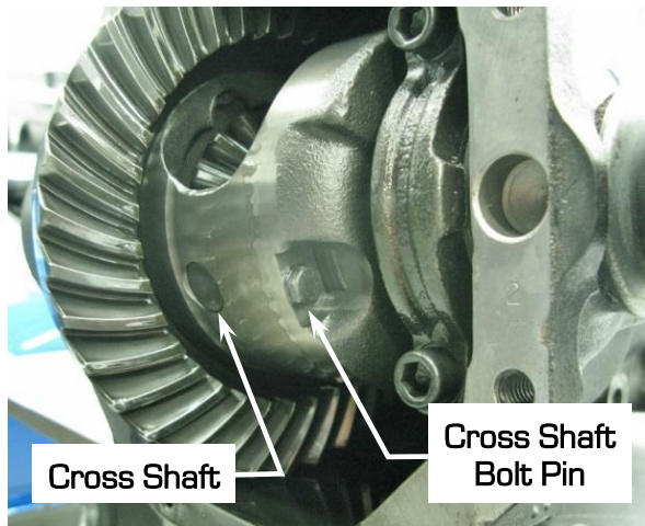
Figure 69 - Cross Shaft & Cross Shaft Bolt Pin
