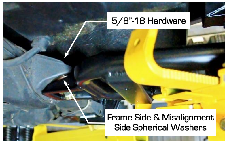
Figure 41 – Bolt Lower Cradle to Frame
