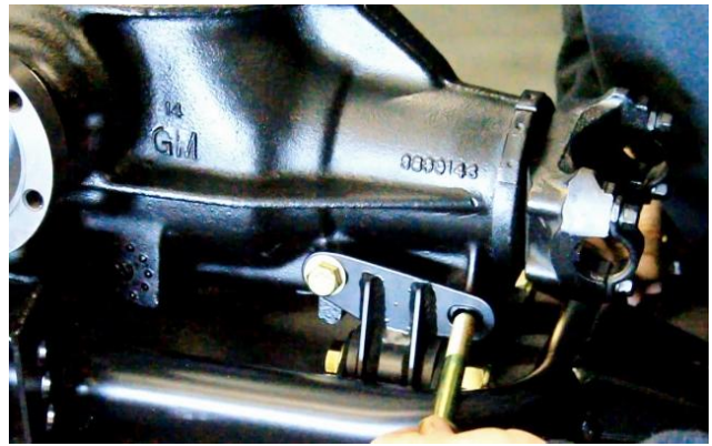
Figure 79 - IRS Lower Cradle/Rear Differential Assembly
