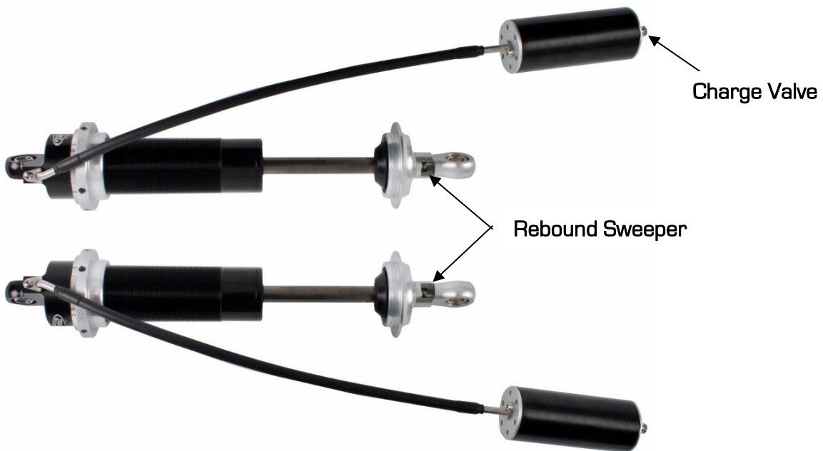
Figure 118a- Detroit Speed Single Adjustable Shock
