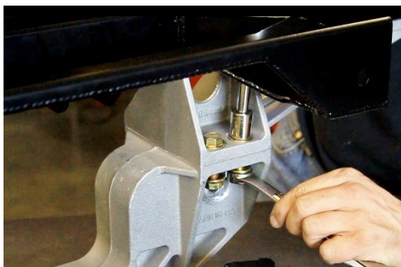
Figure 39 – Assemble the IRS Cradle
