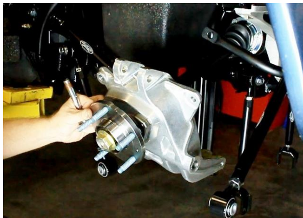
Figure 103 – Install Rear Upright to Outer CV Joint
