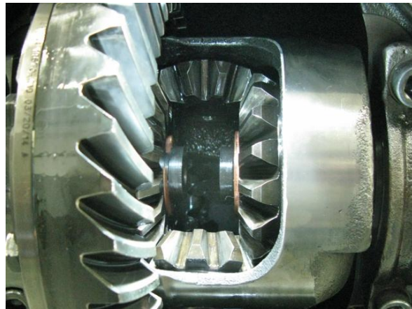
Figure 74 - Install Detroit Speed Stubs Axles
