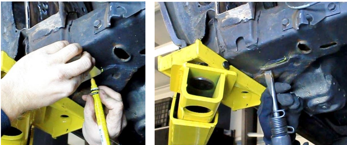
Figure 26 - Trim Frame Gusset
