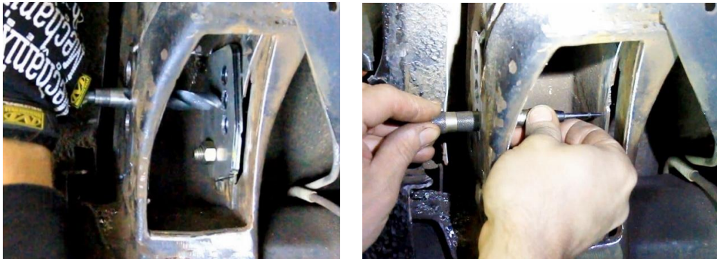
Figure 17 - Center Drill Inner Frame Rail
