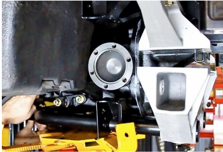
Figure 88 - Install 5/8"-18 Hardware
