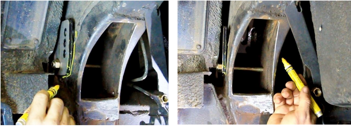
Figure 9 – Trace Outer and Inner Frame Doubler Plates
