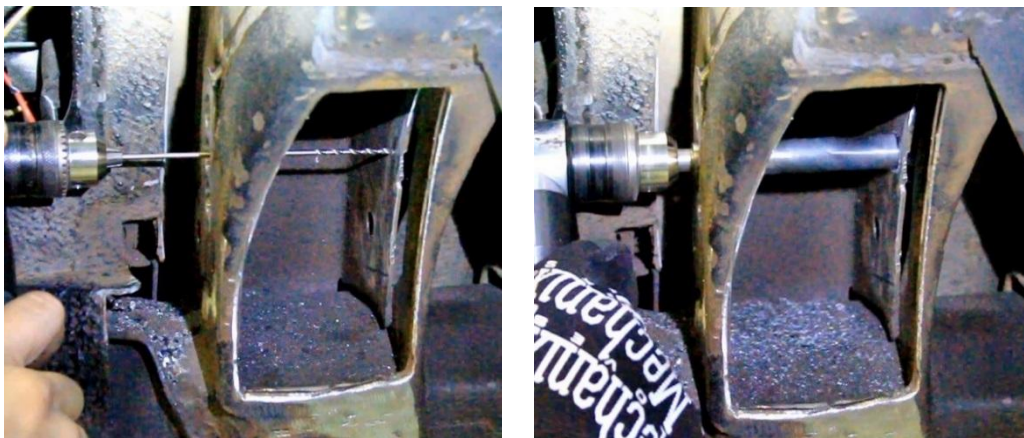
Figure 18 - Drill Inner Frame Rail
