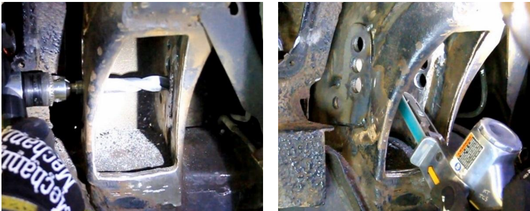
Figure 21 – Drill Upper & Lower Link Holes
