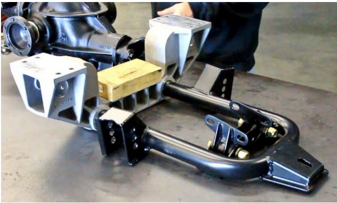
Figure 79 - IRS Lower Cradle/Rear Differential Assembly
