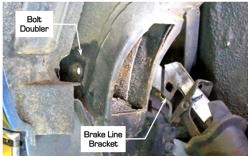
Figure 5 – Remove Park Brake Cable Bracket and Trailing Arm Bolt Doubler
