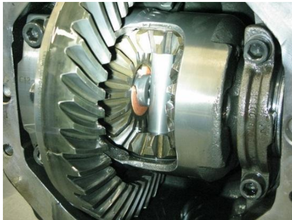
Figure 68 – Remove the Rear Cover
