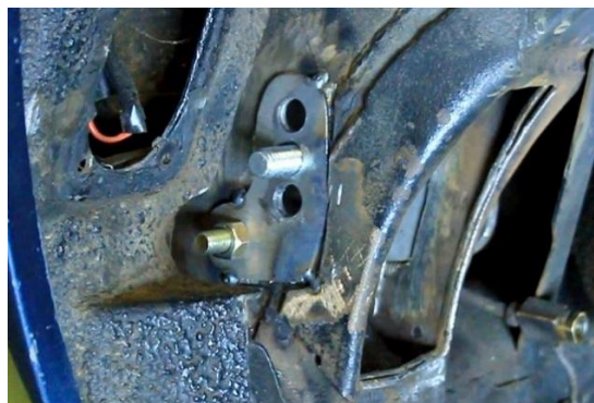
Figure 19 - Locate Inner Doubler Plate
