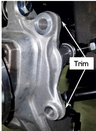
Figure 115 – Trim Upright
