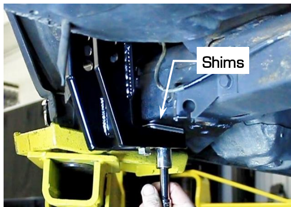
Figure 33 - Install Trailing Arm Bracket Assembly
