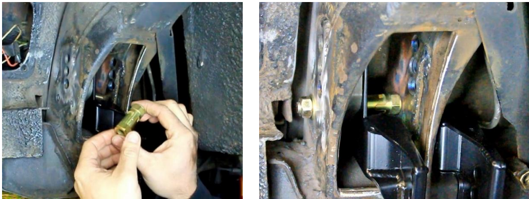
Figure 23 - Trailing Link Bracket
