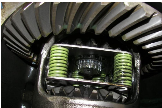
Figure 71 - Remove Snap Rings
