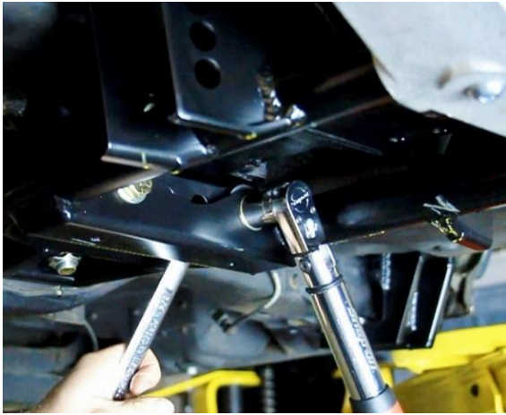
Figure 93 – Torque Lower Differential Bracket
