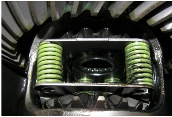
Figure 73 - Remove Stock Stub Axles
