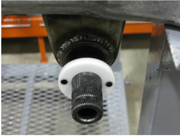
Figure 13- Installing the Bushing & Sway Bar
