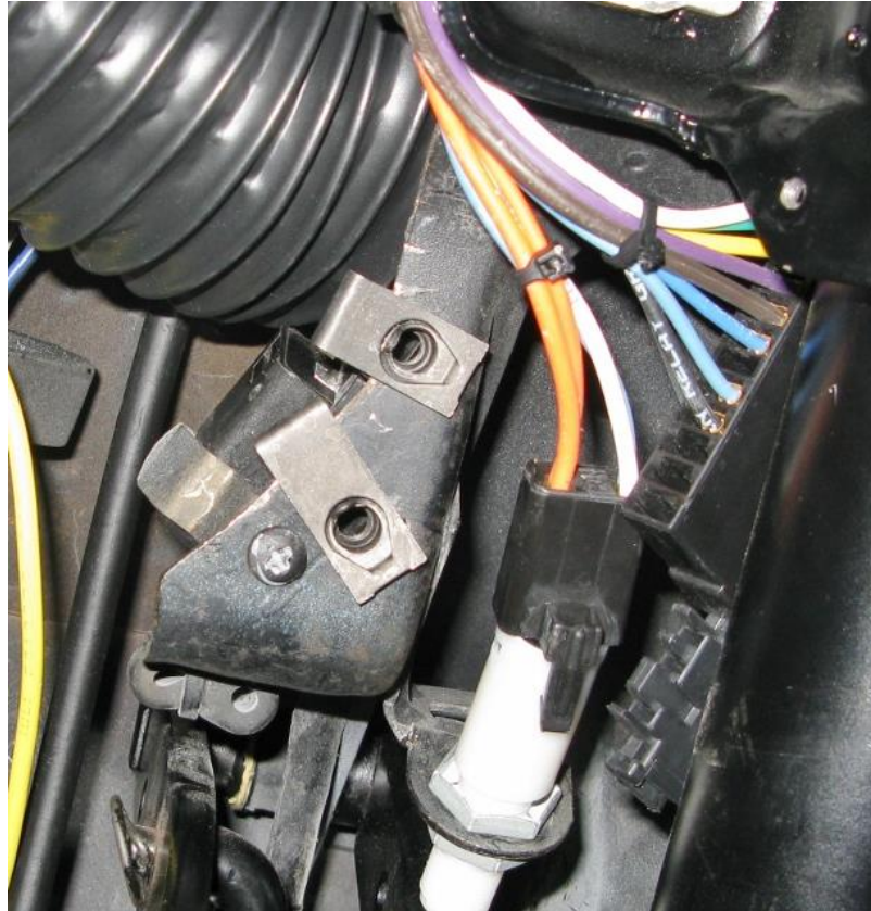
Figure 13 - Install U-nuts
