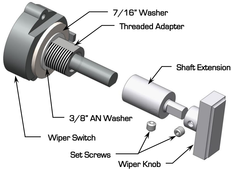
Figure 4 - 1968 Chevelle Wiper Switch Assembly
