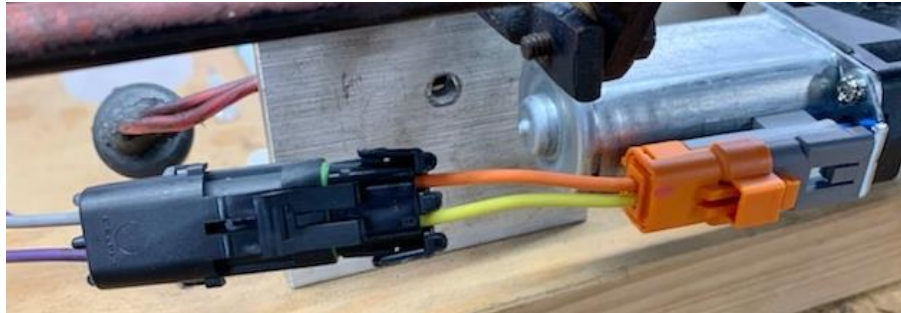
Figure 39 - Connect Harness
