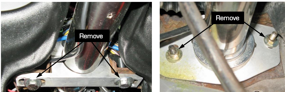
Figure 17 - Remove Steering Column Hardware
