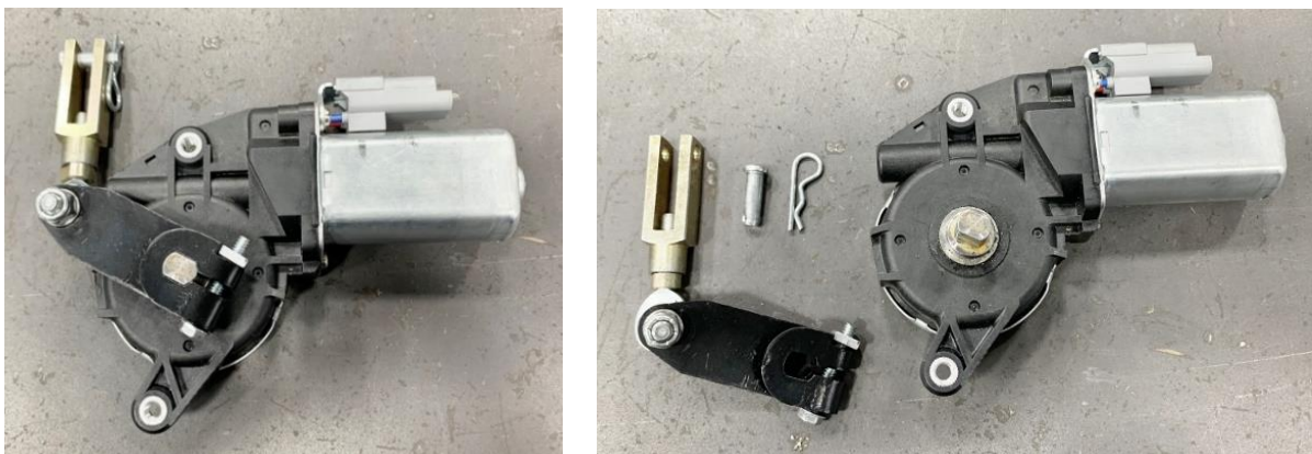
Figure 34 - Remove Pitman Arm
