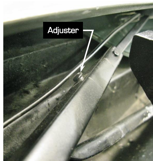
Figure 46 - Adjuster Screw
