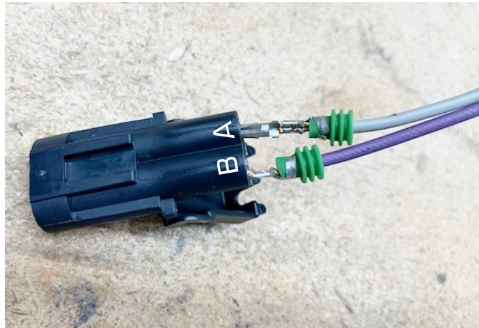
Figure 26 - Wiper Door Motor Terminals
