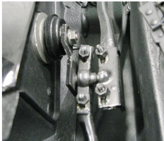
Figure 7 - Remove Wiper Linkage
