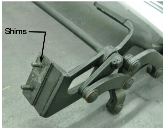
Figure 6 - Wiper Door Shims
