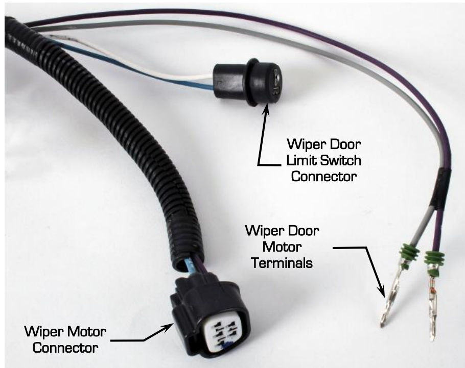
Figure 23 - Wiper Door Terminals, Wiper Motor & Limit Switch Connectors
