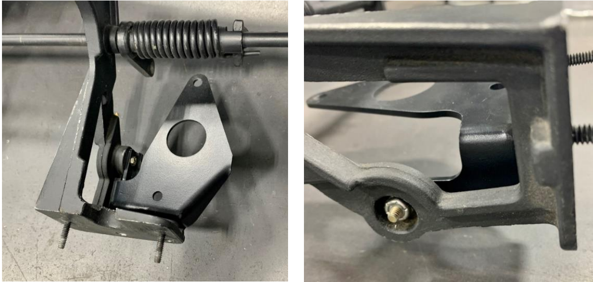
Figure 30 - Install Wiper Motor Bracket
