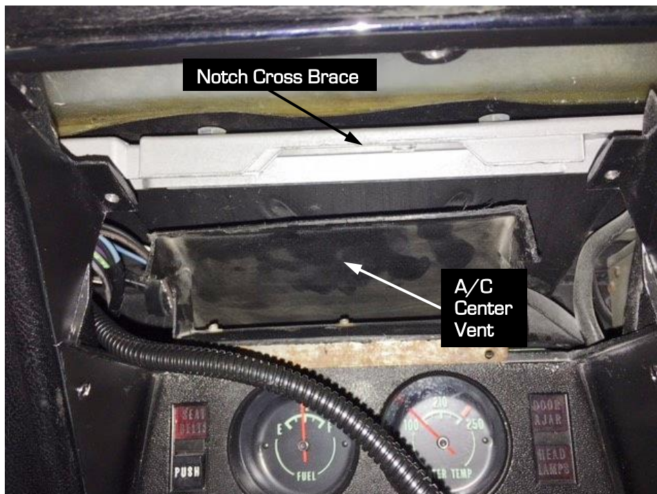
Figure 15 – 1968-69 C3 Cross Brace
