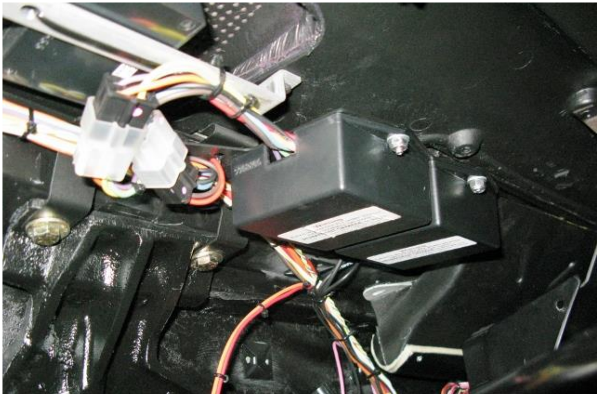
Figure 22 - Mount Wiper Module (Headlight Module also Shown)
