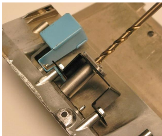
Figure 13 – Drill Center Dash Bezel
