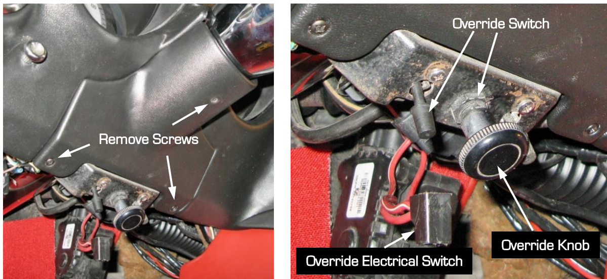
Figure 16 - Remove Lower Column Cover
