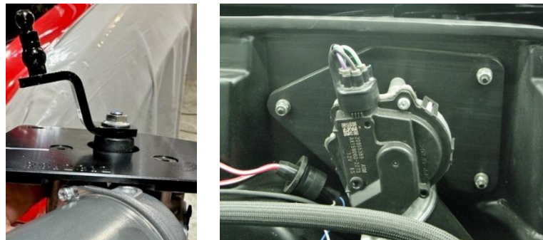
Figure 9 – Attach Wiper Motor to Firewall
