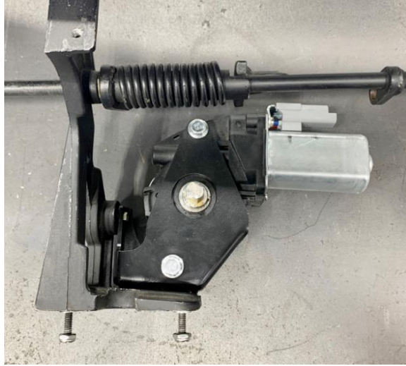
Figure 35 - Install Wiper Door Motor
