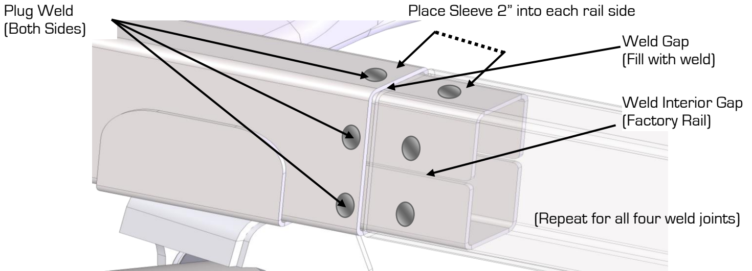
Figure 2 - Frame Rail Doubler Sleeve Final Installation
