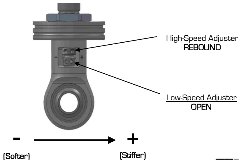
Figure 22b – Detroit Speed Recommended Settings
