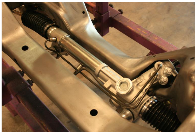
Figure 5 – Installed Rack
