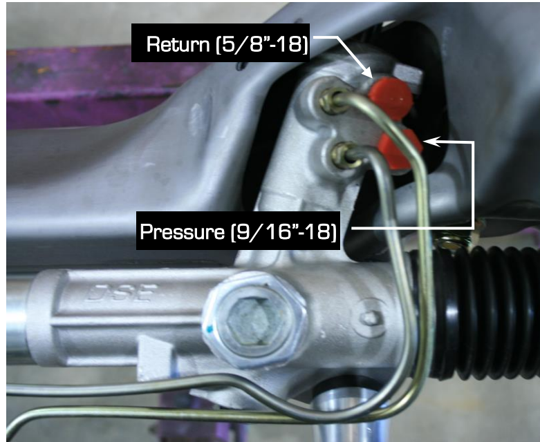
Figure 18 - Pressure and Return Port Locations
