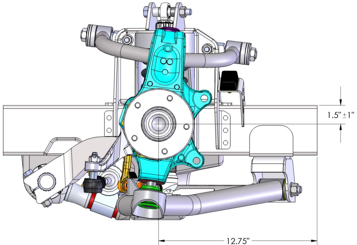
Figure 1 - X-Gen Wheel Centerline Location
