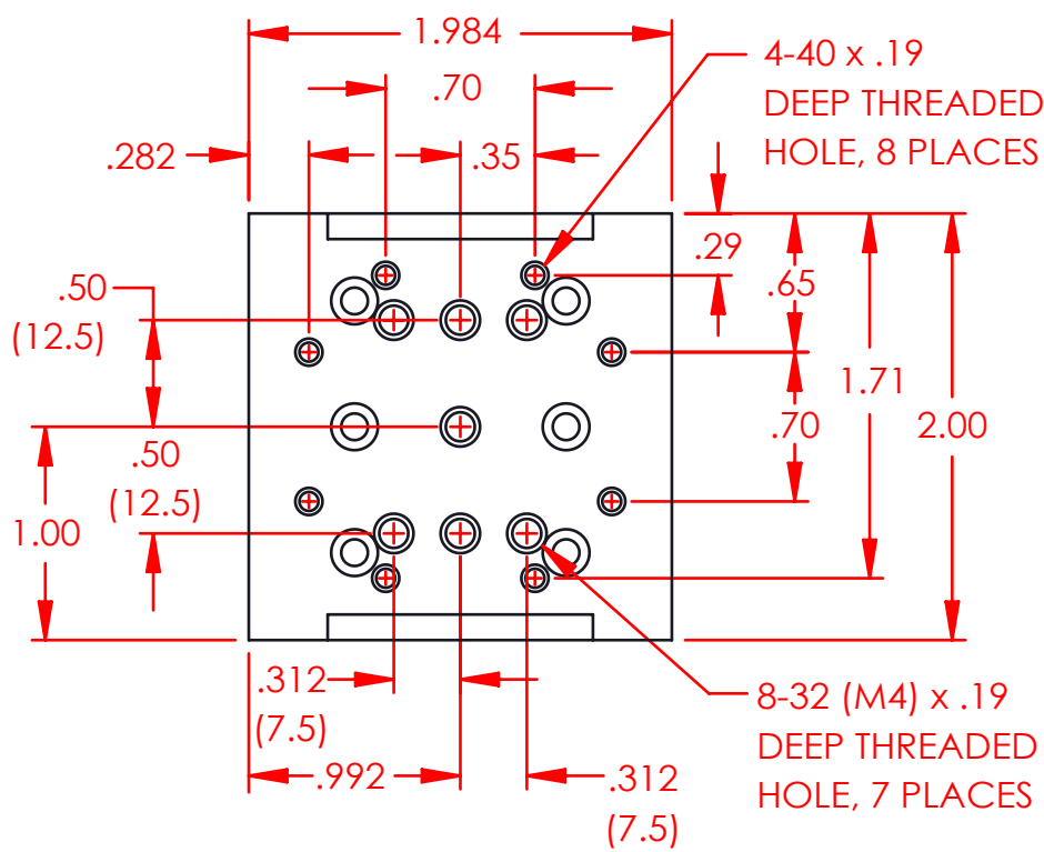
TOP PLATE
