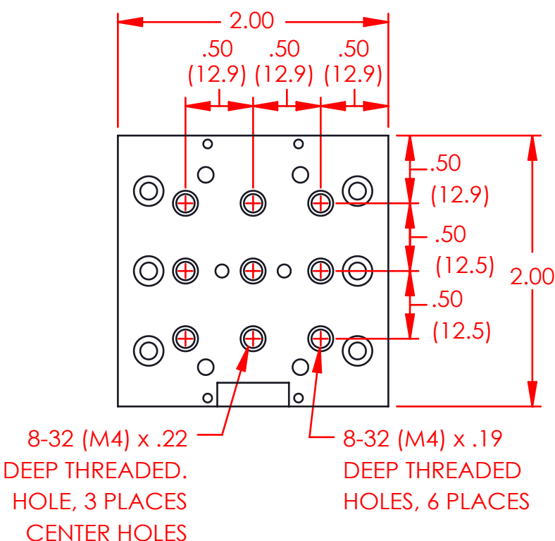
BASE PLATE
