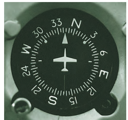
Figure 1-27 Heading indicator.
