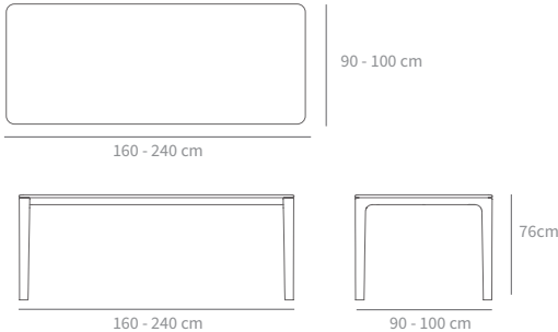
H 76 W 160, 180, 200, 220, 240 D 90, 100 CM
