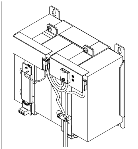
Fig. 14-3 Isometric view
