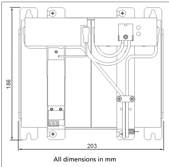
Fig. 14-1 Front view
