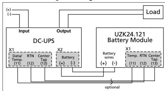
Fig. 4-1 Wiring scheme
