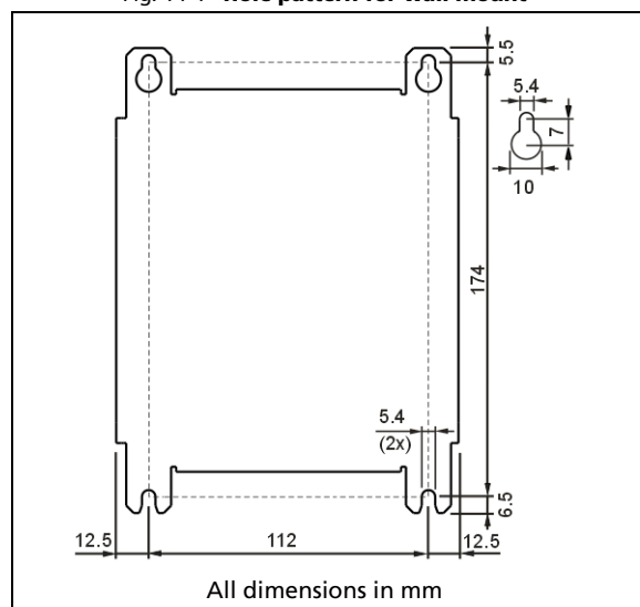
Fig. 14-4 Hole pattern for wall mount
