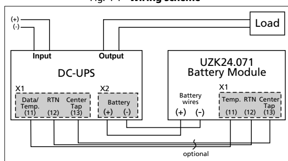
Fig. 4-1 Wiring scheme
