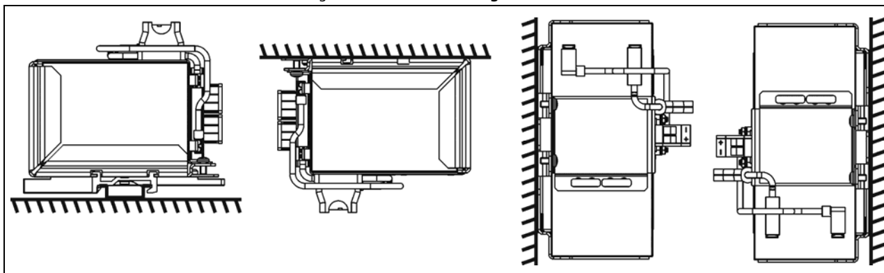
Fig. 18-2 Allowed mounting orientation
