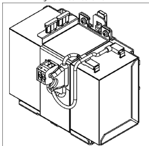
Fig. 15-3 Isometric view
