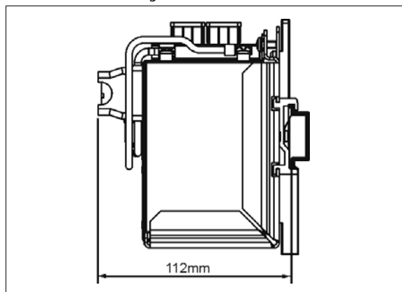
Fig. 15-2 Side view
