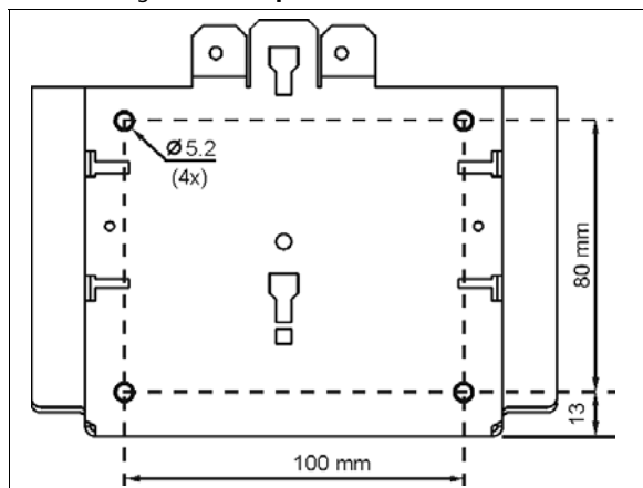
Fig. 16-2 Hole pattern for wall mount
