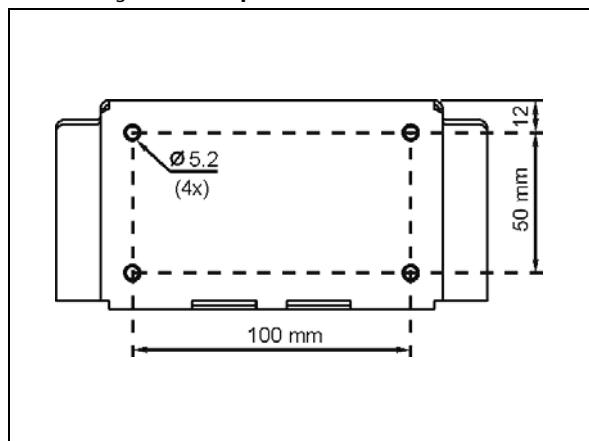
Fig. 16-3 Hole pattern for bottom mount
