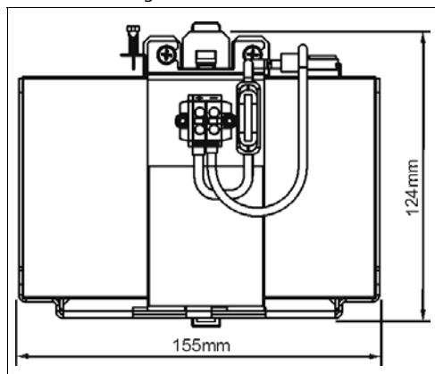
Fig. 15-1 Front view
