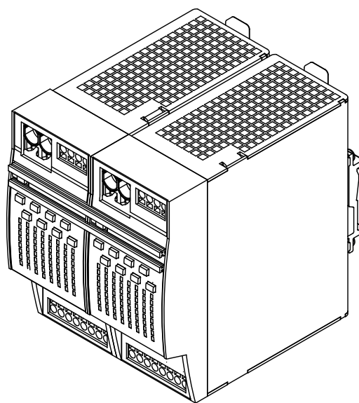
Fig. 23-2: Mounting example
