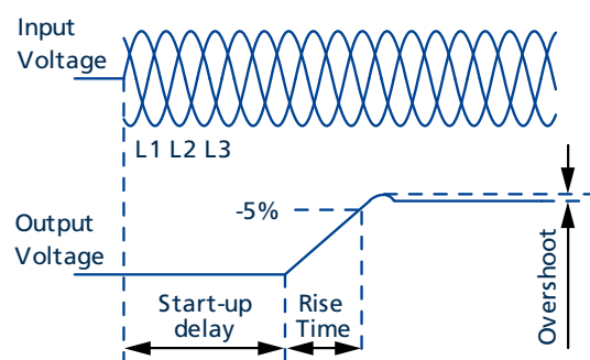
Fig. 3-2: Turn-on behavior, definitions
