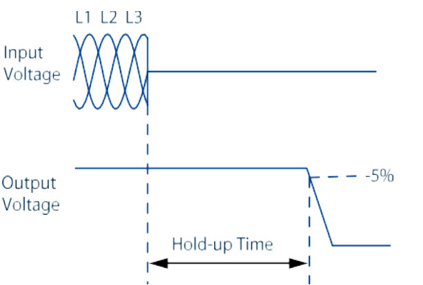
Fig. 7-2: Shut-down behavior, definitions
