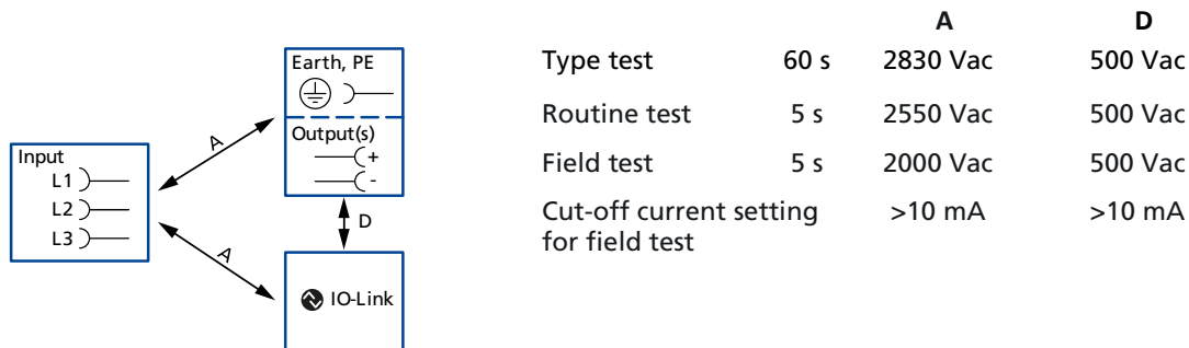
Fig. 18-1: Dielectric strength
