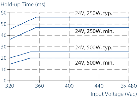
Fig. 7-1: Hold-up time vs. input voltage
