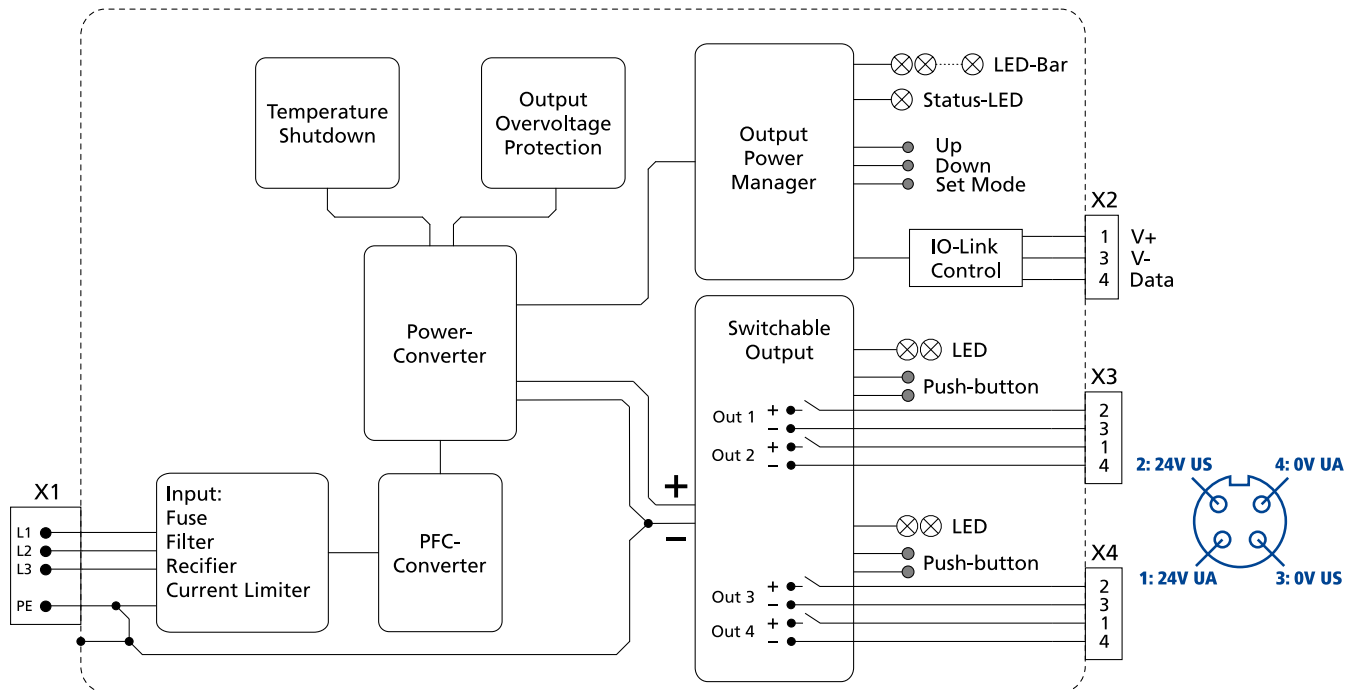
Fig. 12-1: Functional Diagram FPT500.245-018-103
