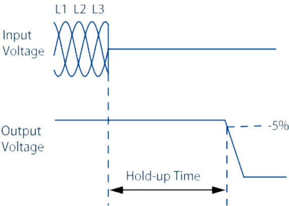
Fig. 7-2: Shut-down behavior, definitions
