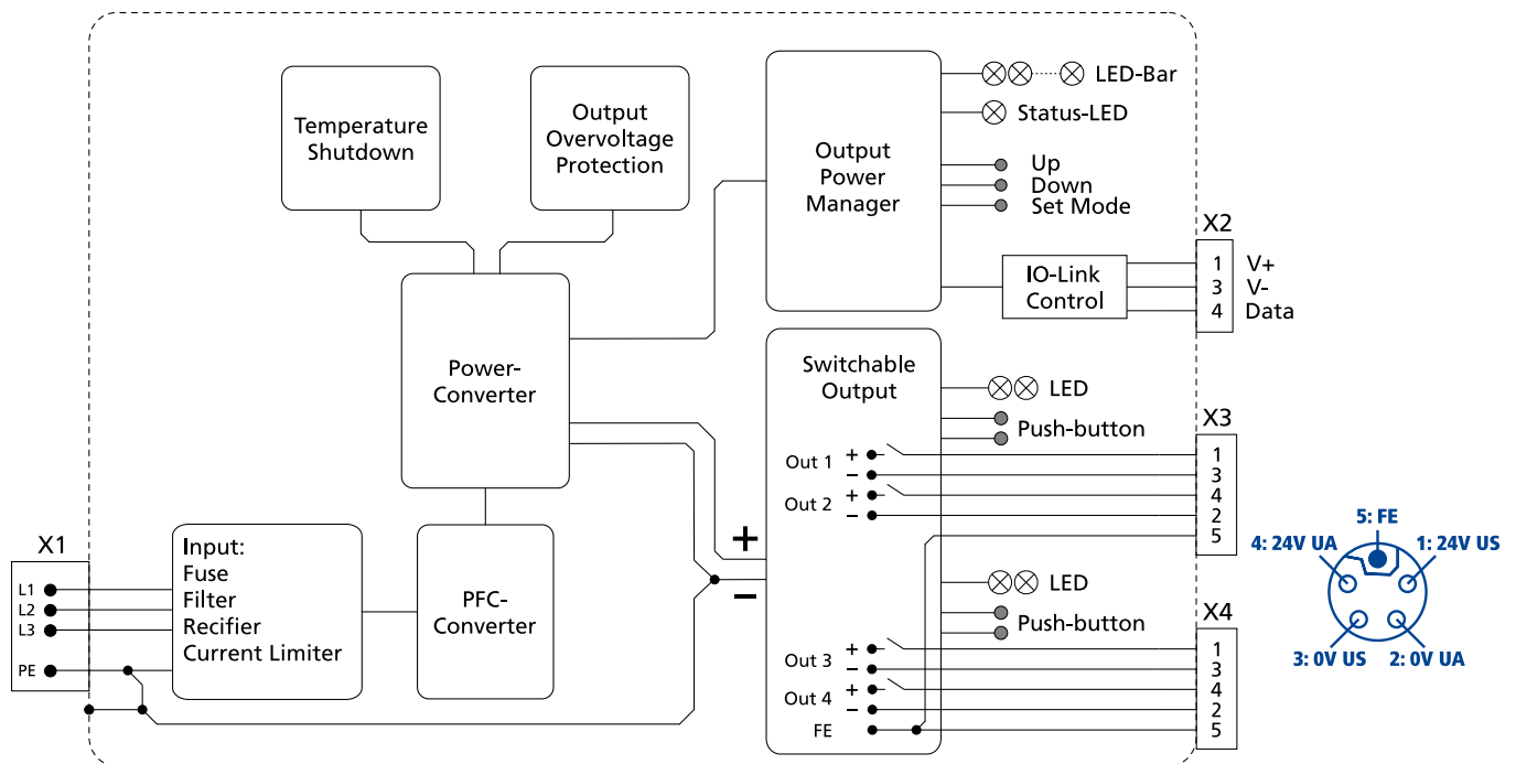
Fig. 12-3: Functional Diagram FPT500.245-034-105
