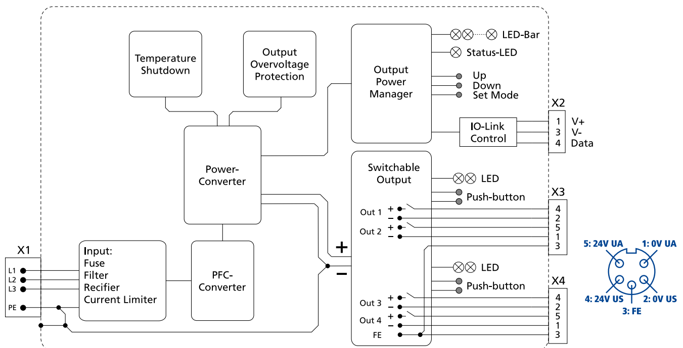
Fig. 12-2: Functional Diagram FPT500.245-062-117
