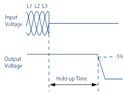
Fig. 7-2: Shut-down behavior, definitions
