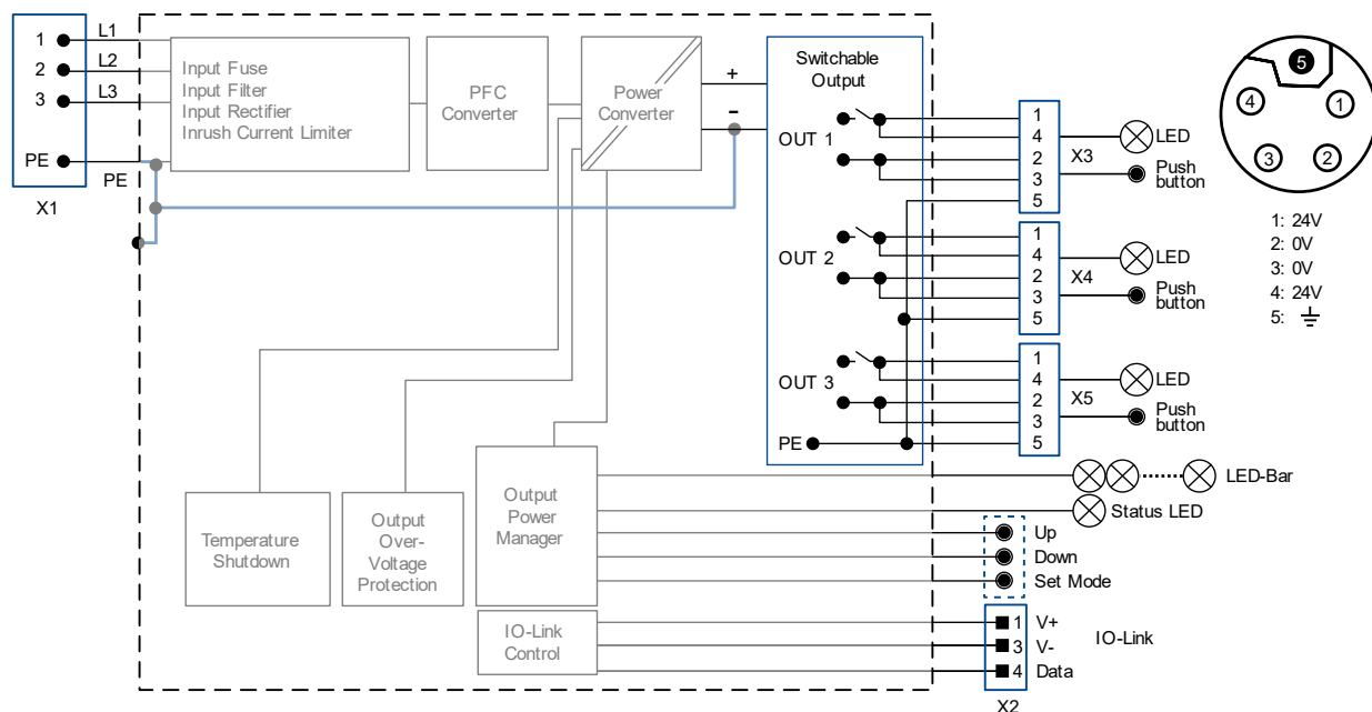
Fig. 12-3: Functional Diagram FPT500.245-036-104
