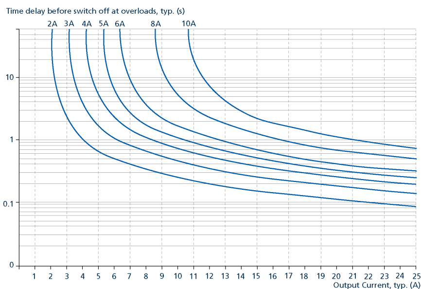
Fig. 6-2: Trip curve diagram for max 10A
