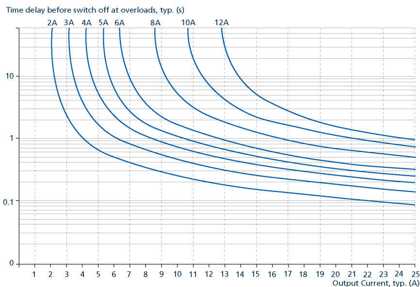
Fig. 6-1: Trip curve diagram for max 12A
