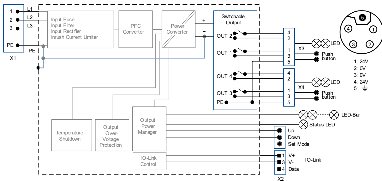
Fig. 12-4: Functional Diagram FPT500.245-034-105
