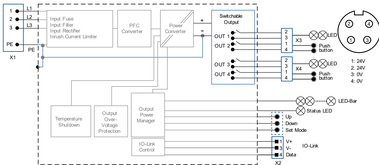
Fig. 12-2: Functional Diagram FPT500.245-018-103
