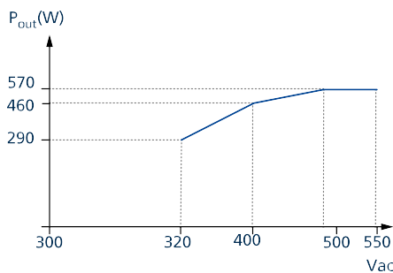
Fig. 23-1: Two phase power capability
