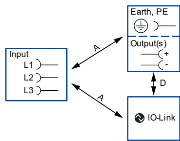
Fig. 18-1: Dielectric strength
