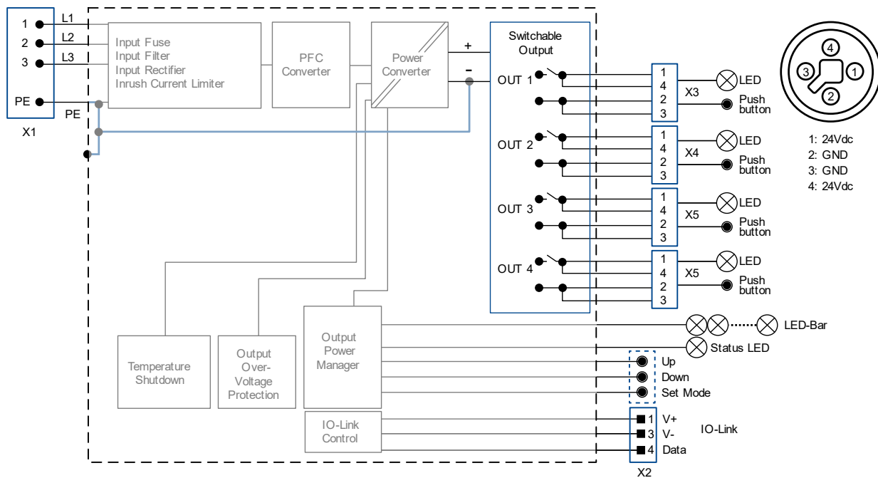
Fig. 12-5: Functional Diagram FPT500.245-044-109
