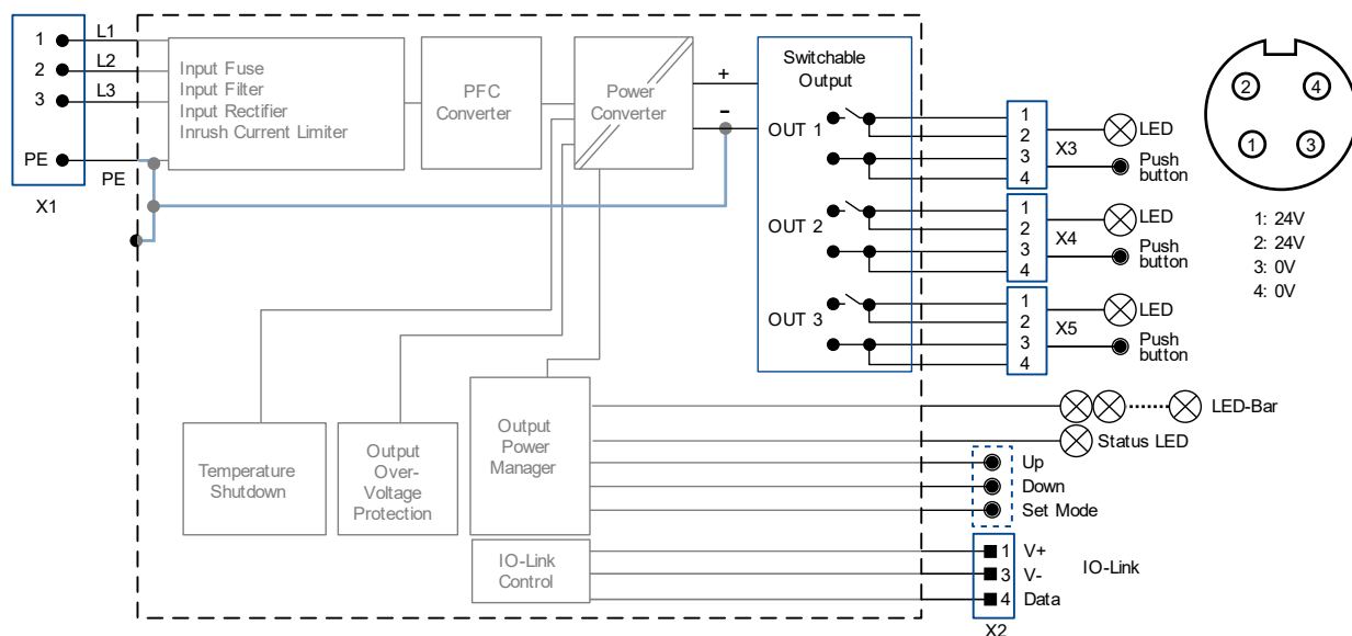
Fig. 12-1: Functional Diagram FPT500.245-020-101
