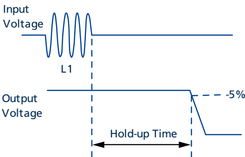
Fig. 7-2: Shut-down behavior, definitions
