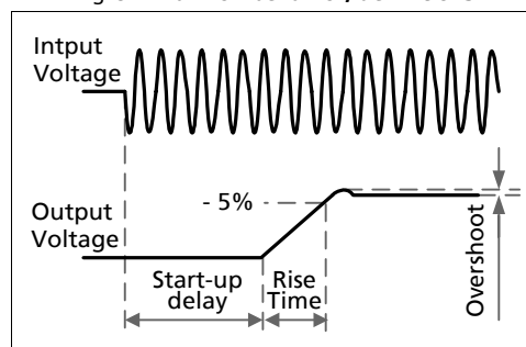
Fig. 5-2 Turn-on behavior, definitions
