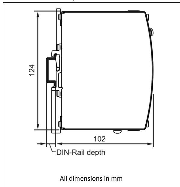
Fig. 21-2 Side view
