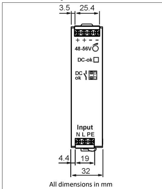
Fig. 21-1 Front view
