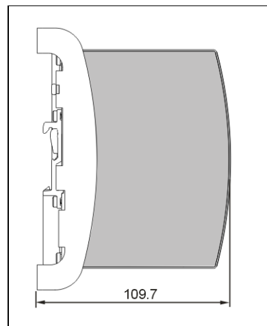
Fig. 22-6 Wall/panel mounting, side view
