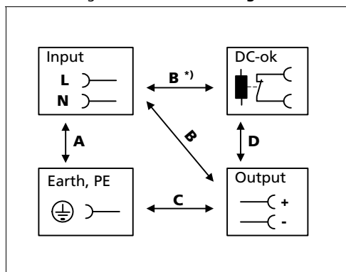
Fig. 20-1 Dielectric strength
