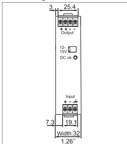
Fig. 20-1 Front view
