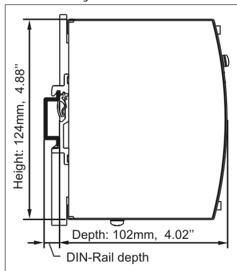
Fig. 20-2 Side view
