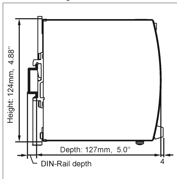
Fig. 16-2 Side view
