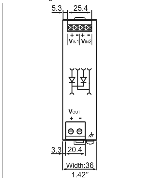
Fig. 16-1 Front view
