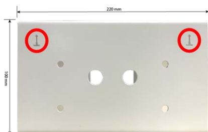
Fig. 9: Dimensions MOBOTIX Q71 Corner/Pole Mount – front view
