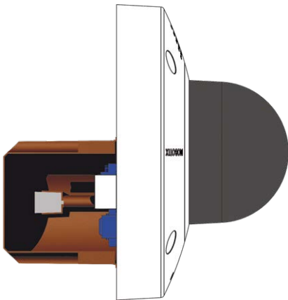
Fig. 5: Side view of MOBOTIX D71 over flush-mounted wall outlet
