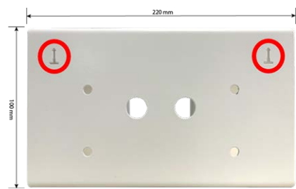
Fig. 9: Dimensions MOBOTIX D71 Corner/Pole Mount – front view
