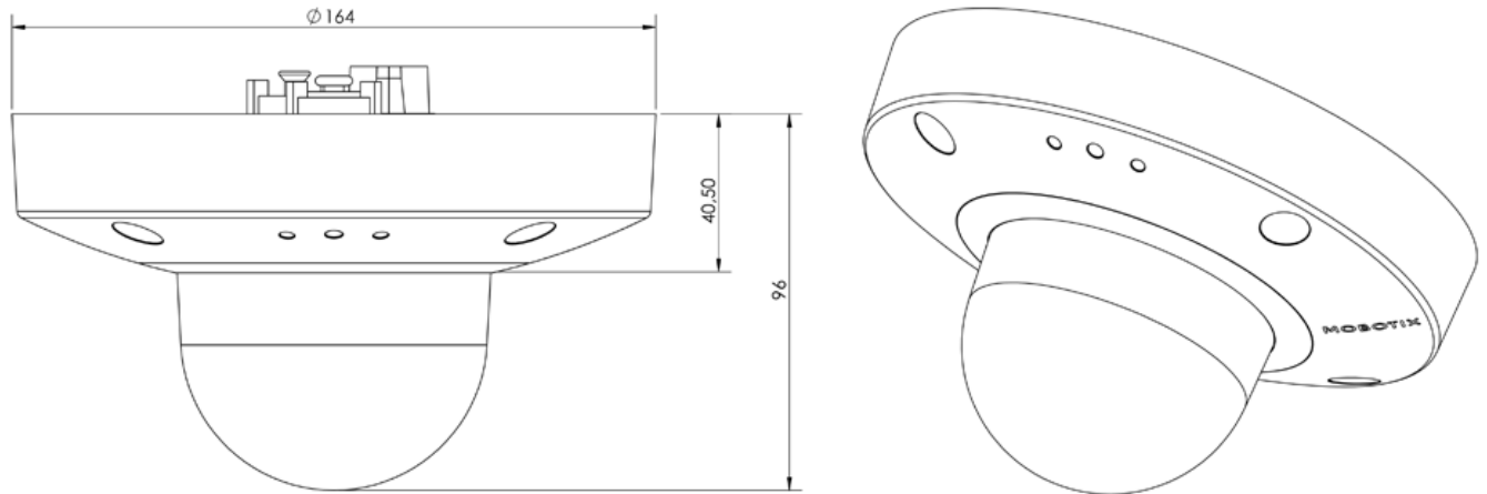
Fig. 4: MOBOTIX D71: All measurements in mm
