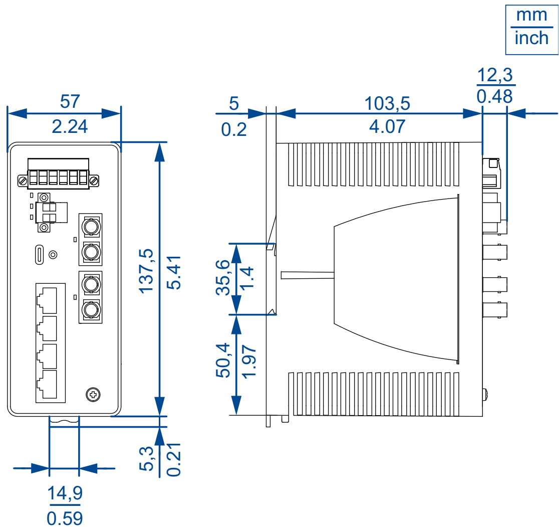
Figure 22: Device variants in narrow plastic casing
