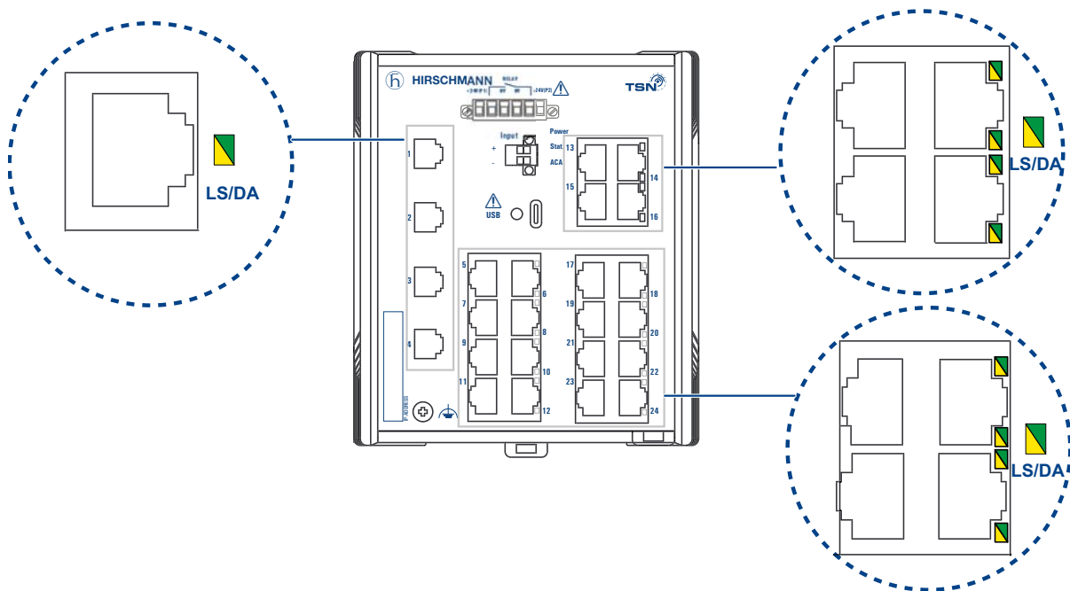
Figure 5: LED display elements for a high port device variant with SFP slots and 20 × RJ45 sockets
