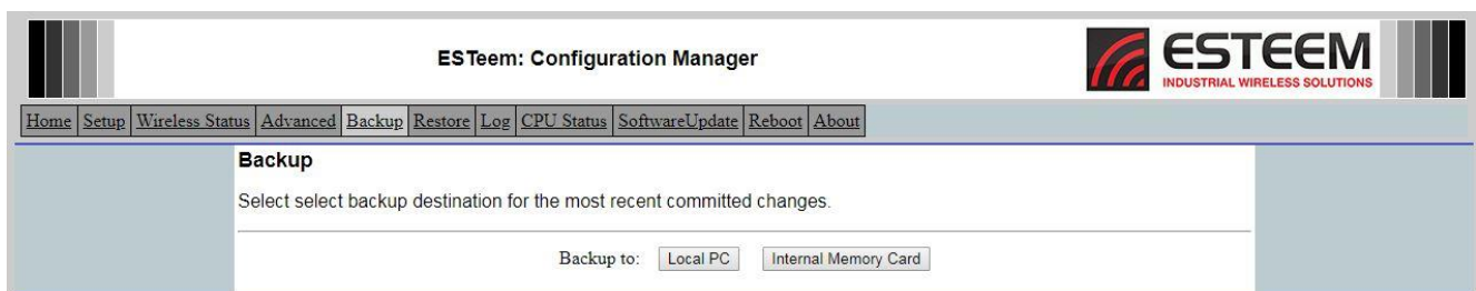
Figure 8: Backup Screen
