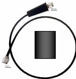
ESTeem Model 195Ep Interface Cable, EST P/N AA241LMR, N-male/TNC-male connectors and Mastic Pad for weatherproofing
