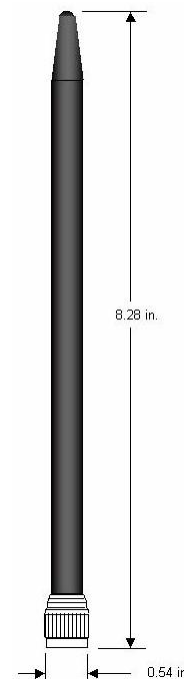
Model AA20DMEp
