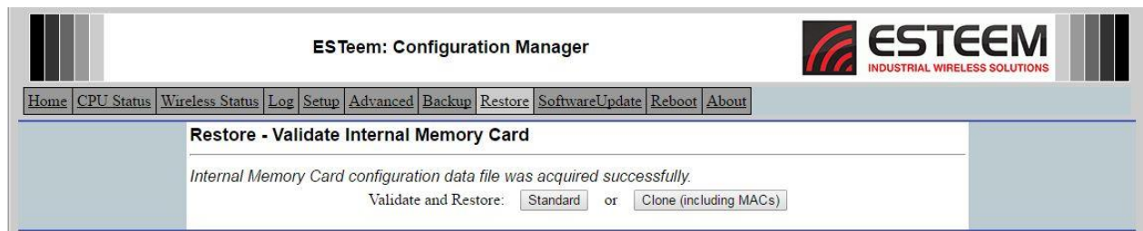
Figure 3: Restore as Clone Option
