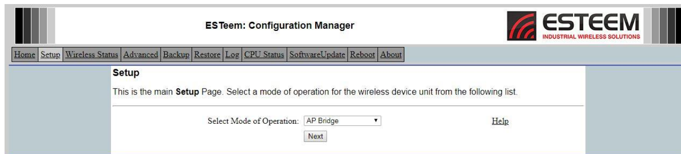
Figure 5: Setup Screen
