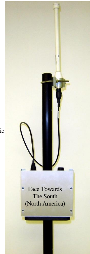
Figure 13: Completed AA195PM Mounts
