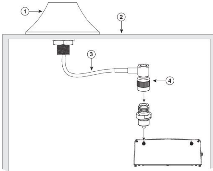
Figure 3: Antenna Detail
