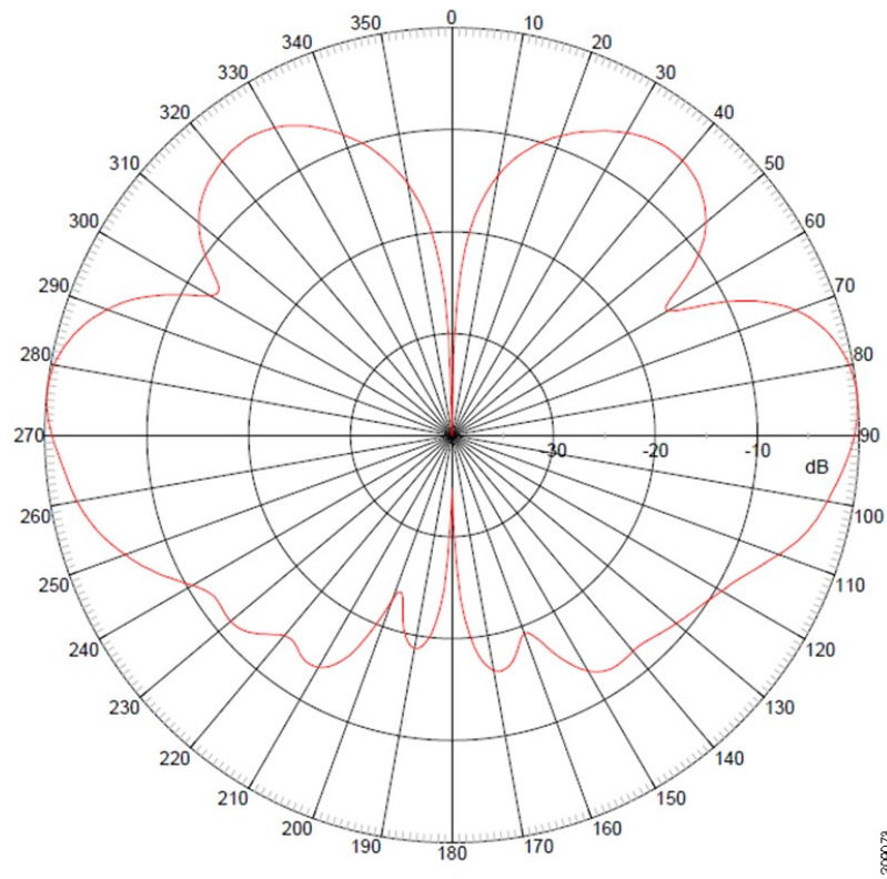
Figure 2: Elevation Radiation Pattern (2.4 GHz)
