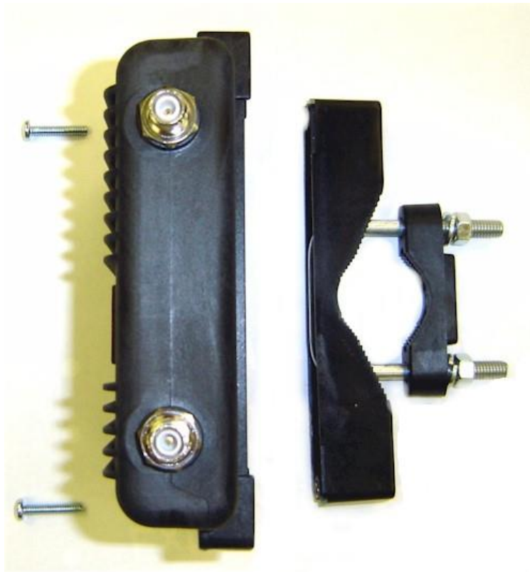
Figure 8: Pole Mount Connection to Case (Heat Shield Removed for Detail)
