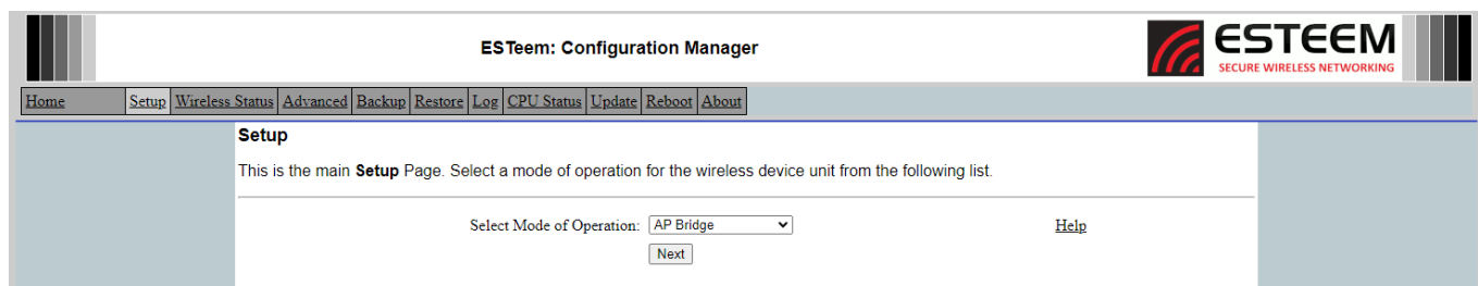
Figure 5: Setup Screen
