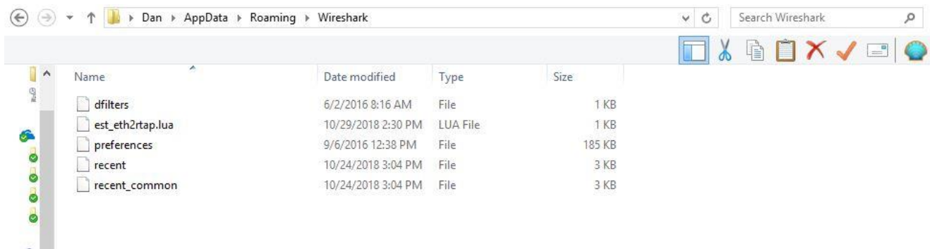
Figure 14: WireShark directory
