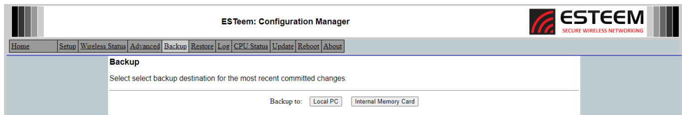
Figure 8: Backup Screen
