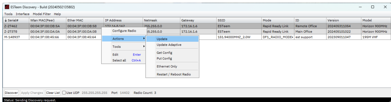
Figure 4: Firmware Update
