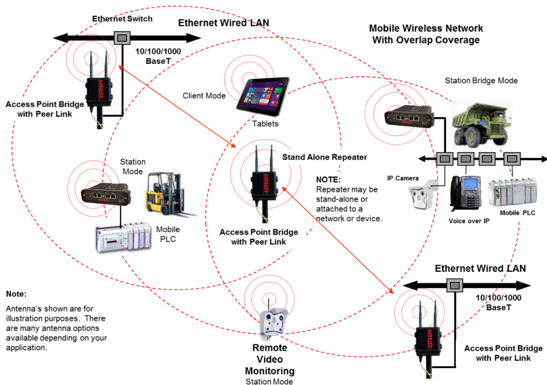
Figure 8: Access Point and Ethernet Bridge
