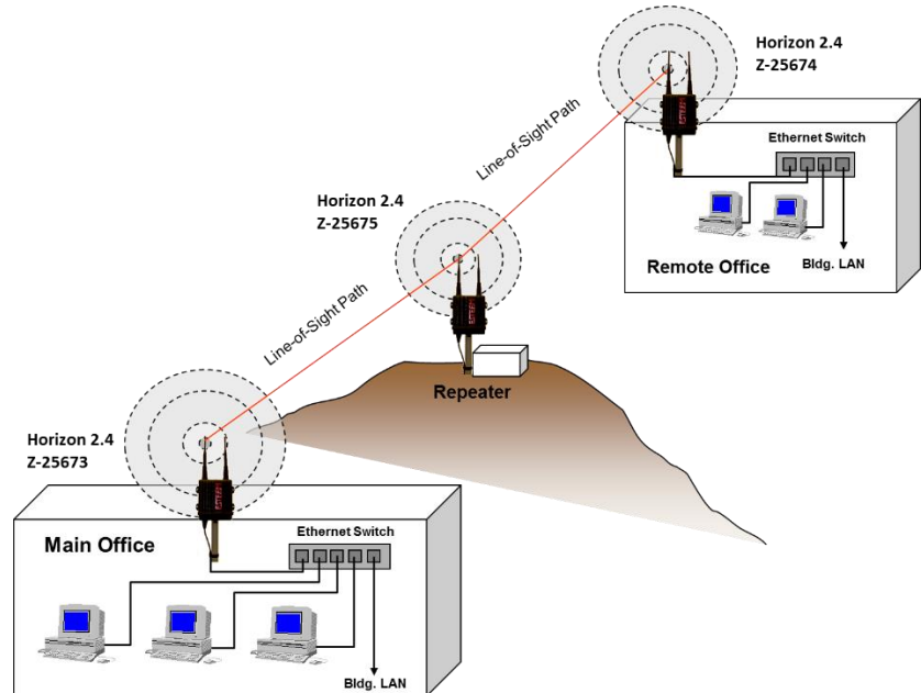
Figure 20: Point to Point Ethernet Bridge with Repeater Example
