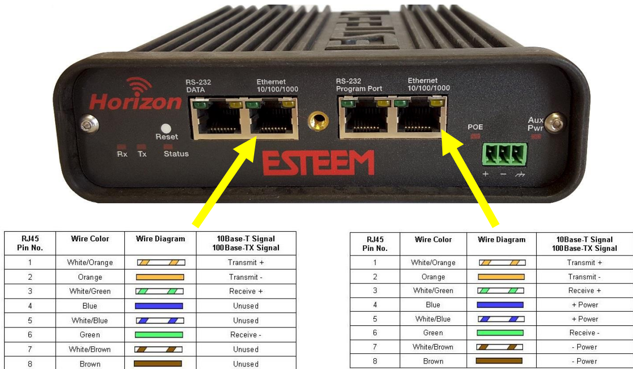
Figure 1: Ethernet Pin Layout
