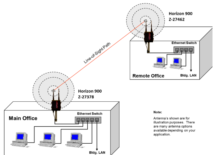
Figure 8: Point to Point Rapid Ready Example
