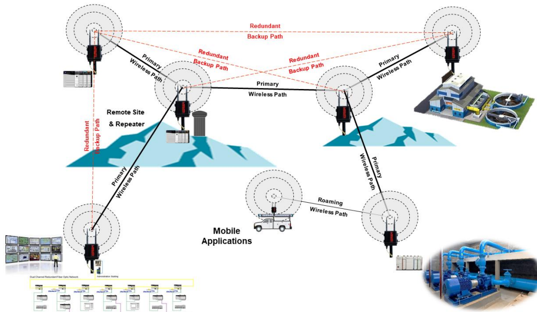
Figure 5: Mesh Network Diagram
