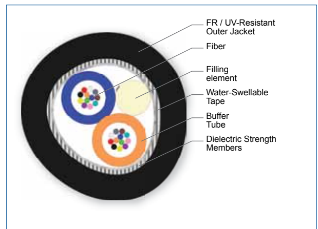
Cross Section of Part Number: 024ESF-T4101D20
